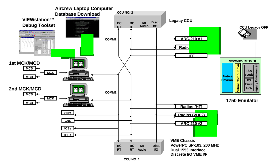
Figure 49. TD-1 Demonstration Configuration
