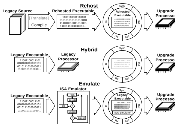
Figure 1. Wrapper Cases
