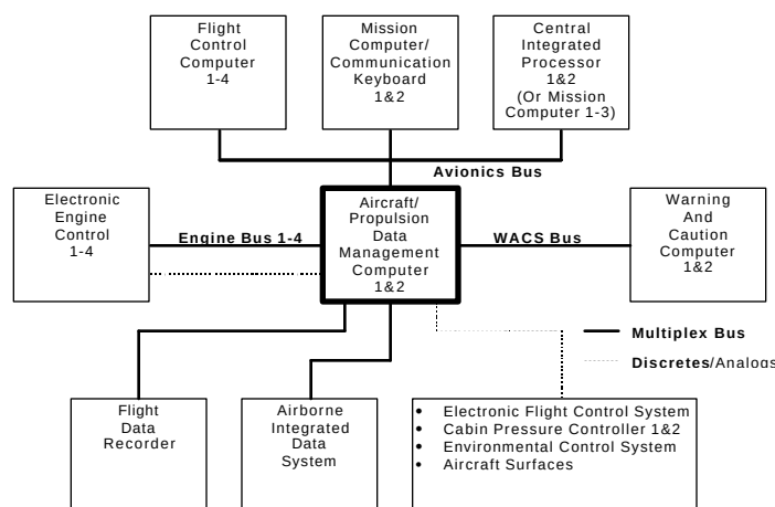
Figure 32. APM Context
