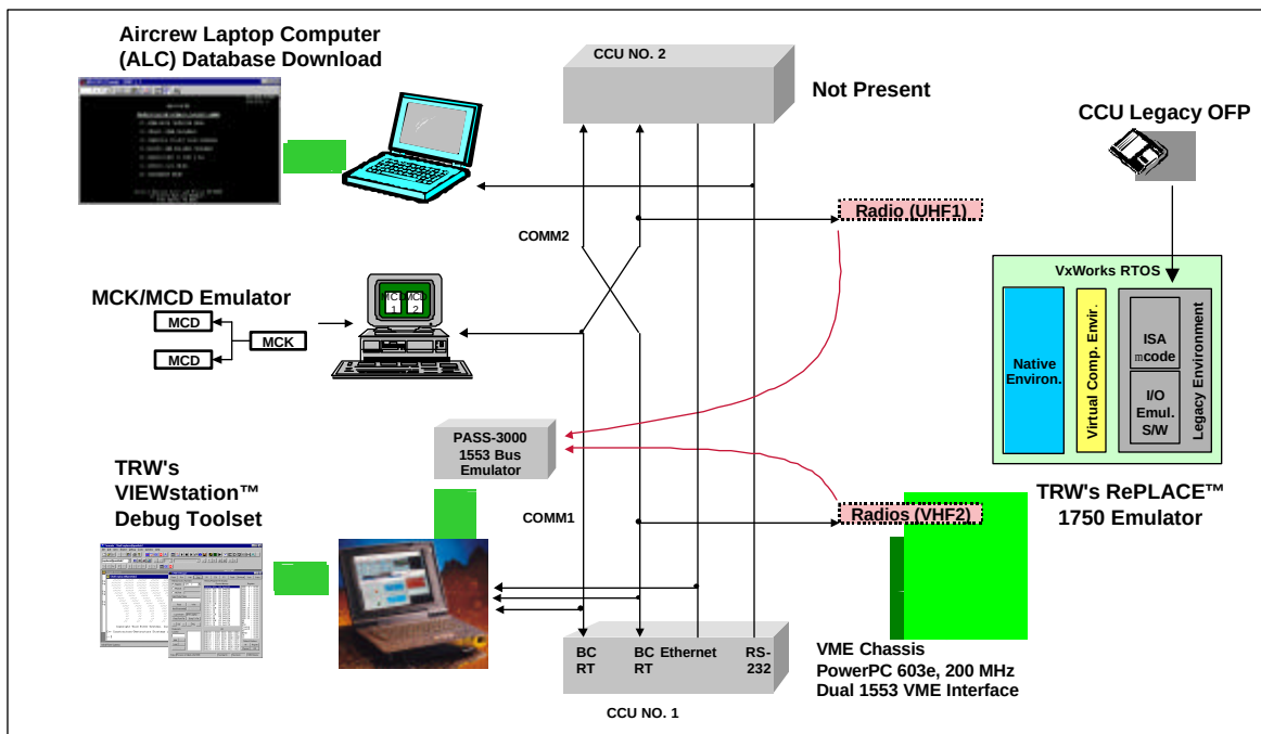
Figure 43. Phase 2 Demonstration Configuration (Physical View)
