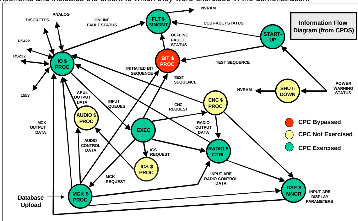
Figure 44. CCU OFP Architecture Components
