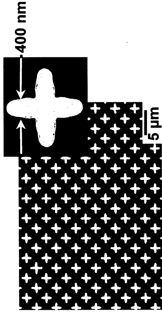
Lift-off; gold on silicon
