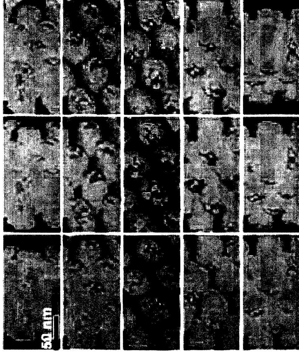
Tomograph of cylinder phase of copolymer blend; 10^\circ rotations. Spontak et al. , Macromol. 29 (1996) 4496
