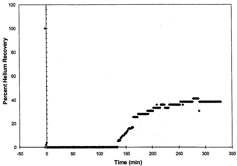
Figure 3a. Helium Recovery Test Site 2 970725
