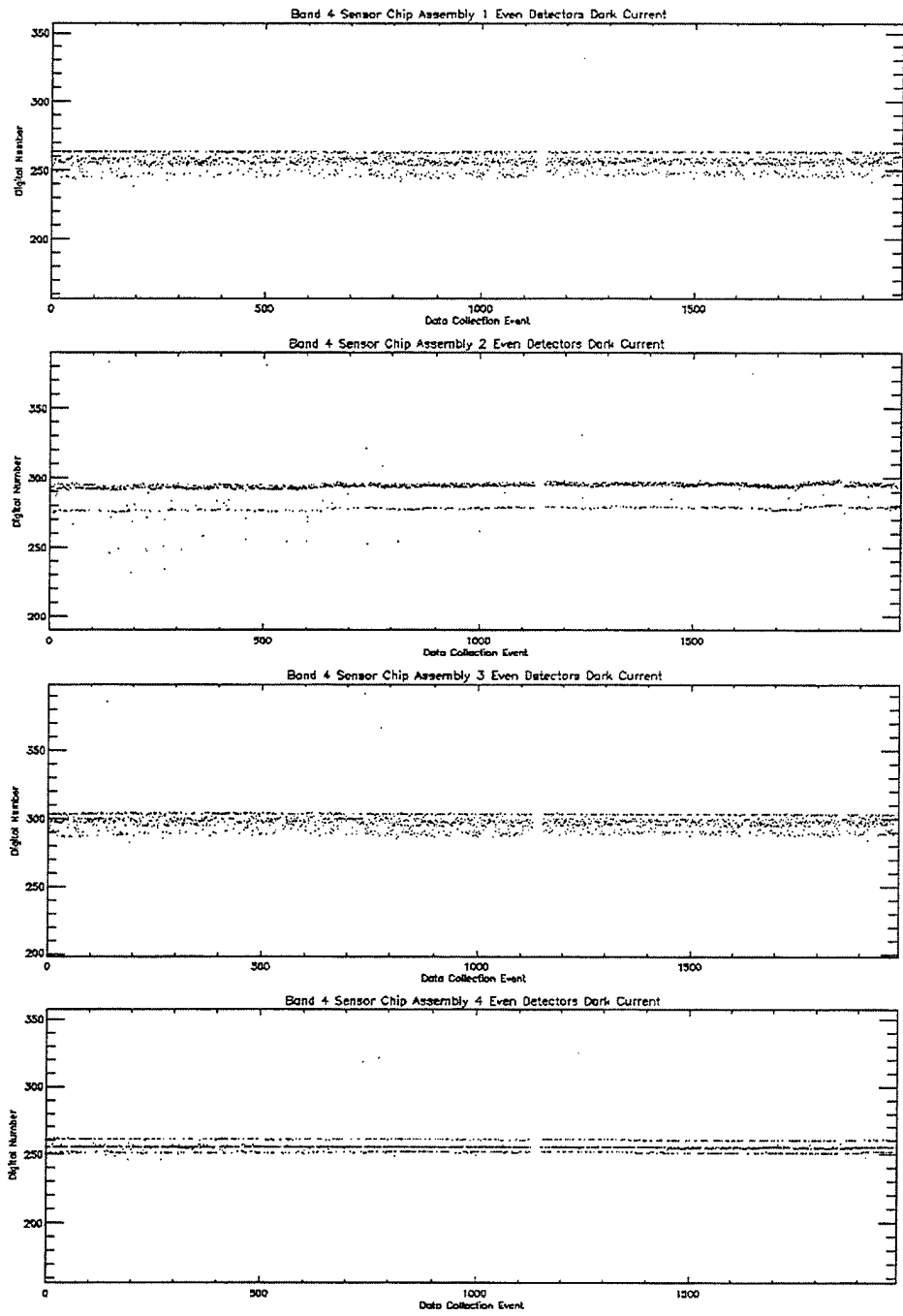
Figure 23. Dark current trending for Band 4 even detectors.
