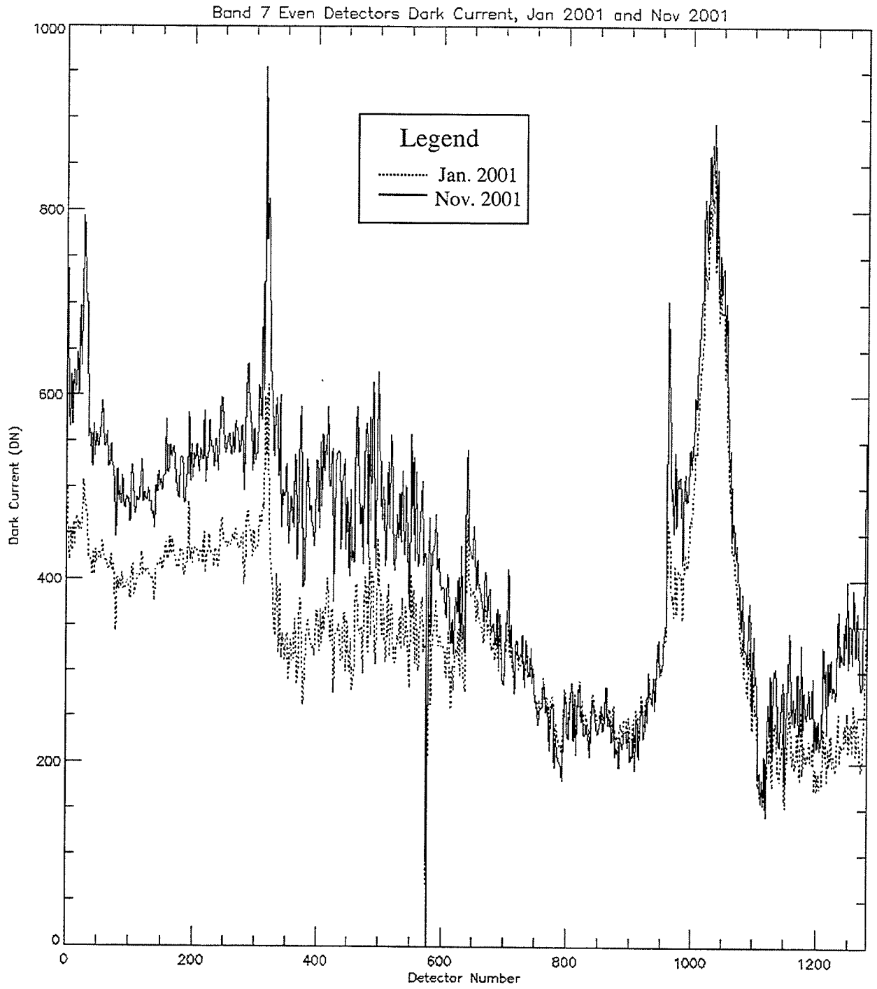
Figure 51. Dark current drifting for Band 7 even detectors between Jan. 2001 and Nov. 2001.
