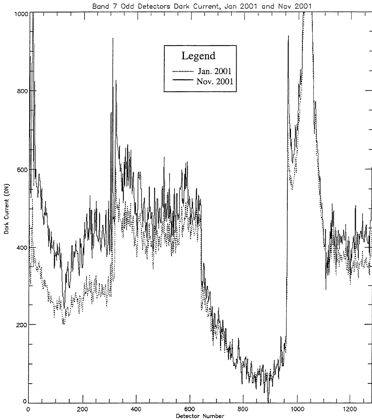
Figure 50. Dark current drifting for Band 7 odd detectors between Jan. 2001 and Nov. 2001.
