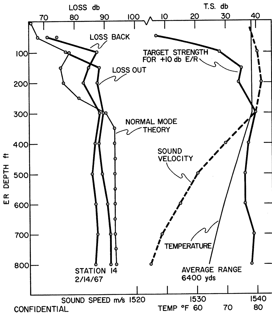
Fig. 11 -- TEMPERATURE AND LOSS PROFILES
