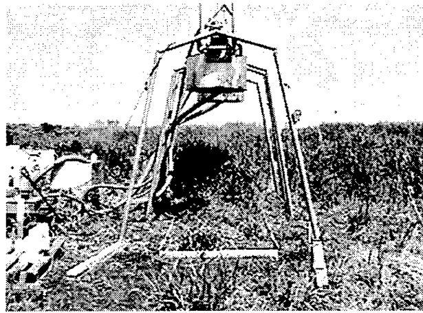
Figure 3. Rainfall simulation on the vegetated dredged material
