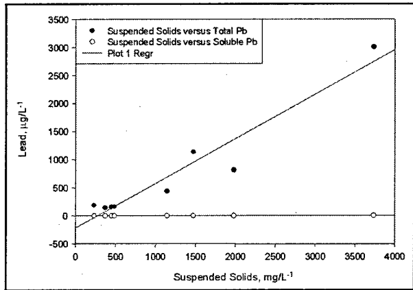
Figure 11. Total and soluble lead versus suspended solids
