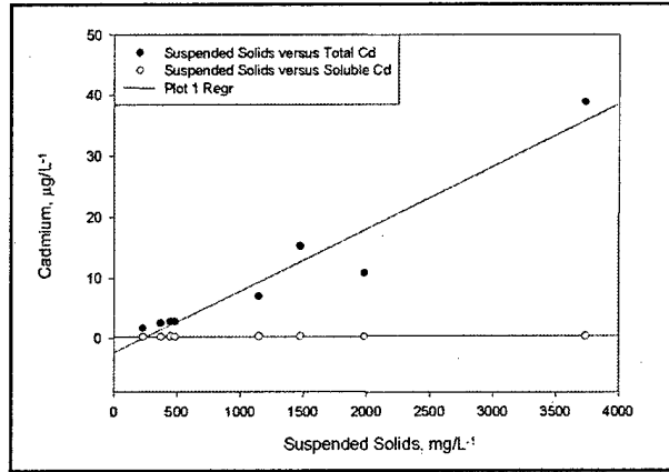
Figure 9. Total and soluble cadmium versus suspended solids
