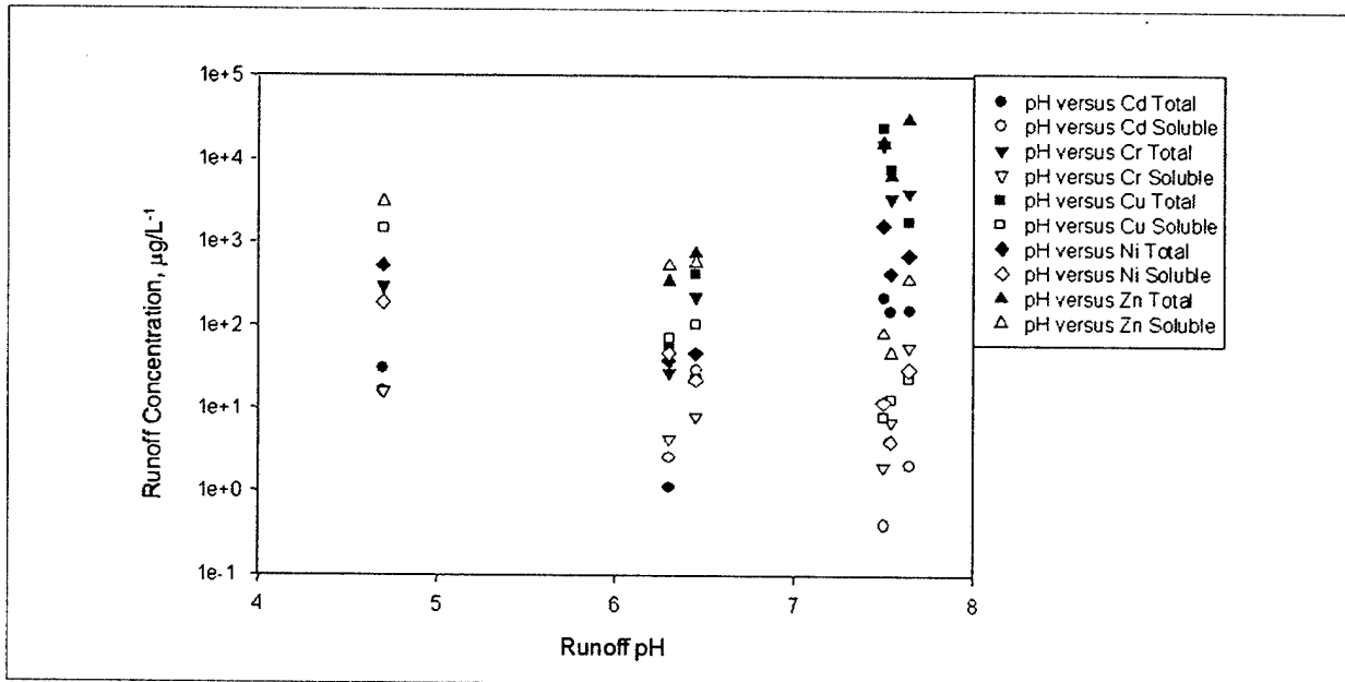
Figure 12. Total and soluble metals versus dredged material pH for Indiana, New Bedford, and Blackrock Harbor sediments
