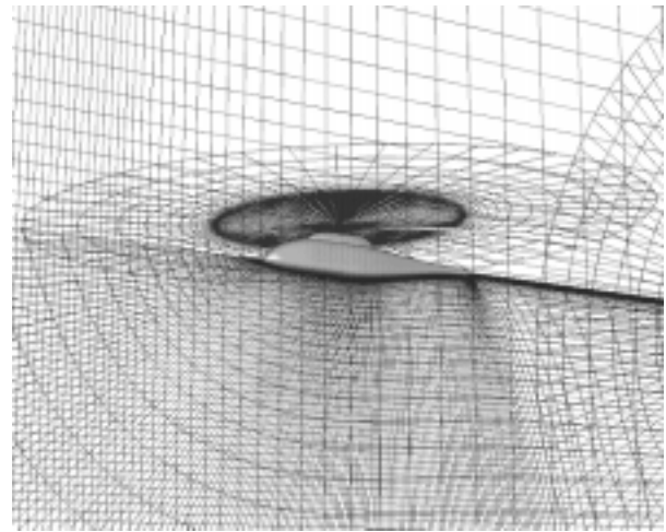
Figure 5: AFDD Grid for ROBIN and Rotor
