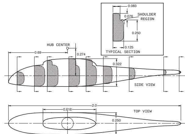
Figure 3: ROtor Body Interaction (ROBIN) fuselage (units of nominal rotor radius)
