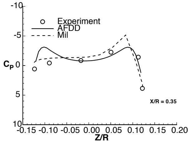
Figure 13: Pressure Comparison at X/R=0.35
