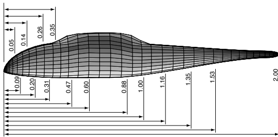
Figure 4: Panels used for Mil fuselage model
