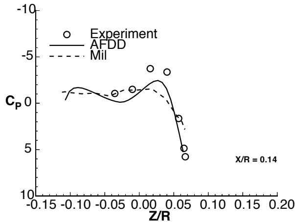
Figure 9: Pressure Comparison at X/R=0.14
