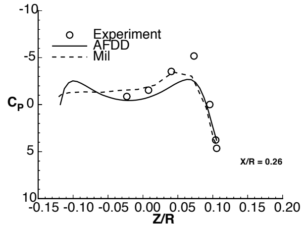
Figure 11: Pressure Comparison at X/R=0.26
