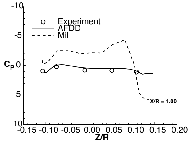
Figure 17: Pressure Comparison at X/R=1.00
