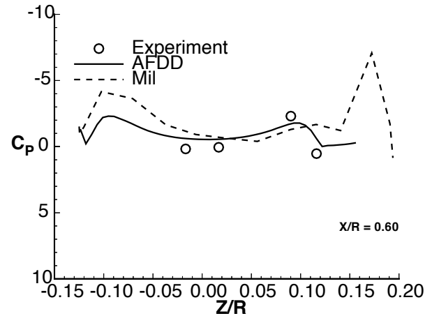
Figure 15: Pressure Comparison at X/R=0.60
