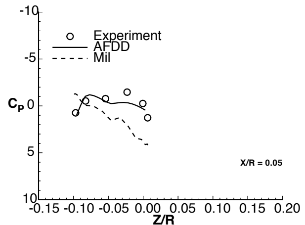
Figure 7: Pressure Comparison at X/R=0.05
