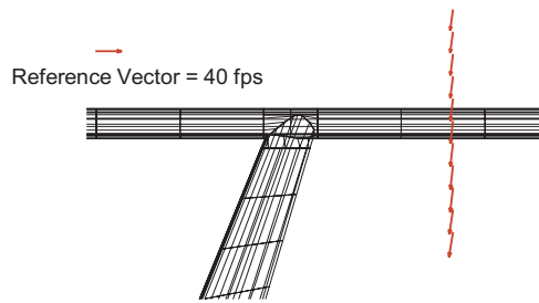
(a) \mu = 0.05 . Average sidewash angle is 11 degrees.
