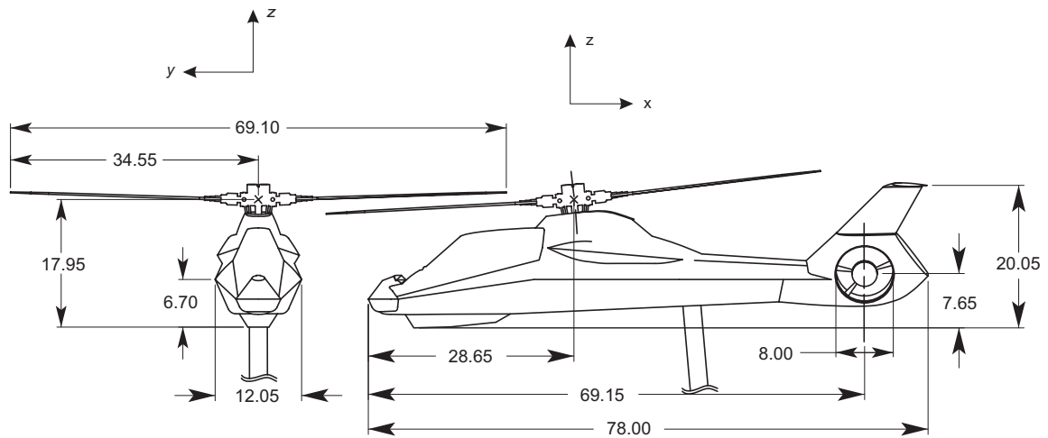
Figure 3. Description of fuselage. All dimensions in inches.
