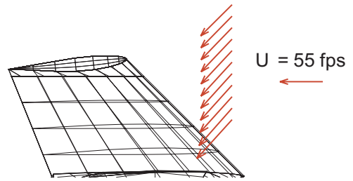
(b) \mu = 0.07 . Average downwash angle is 47 degrees.
