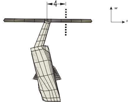
(b) Rear view of horizontal tail measurement locations.
