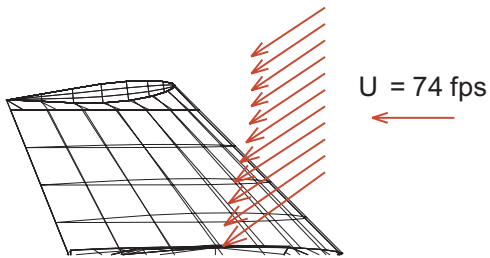
(c) \mu = 0.10 . Average downwash angle is 35 degrees.
