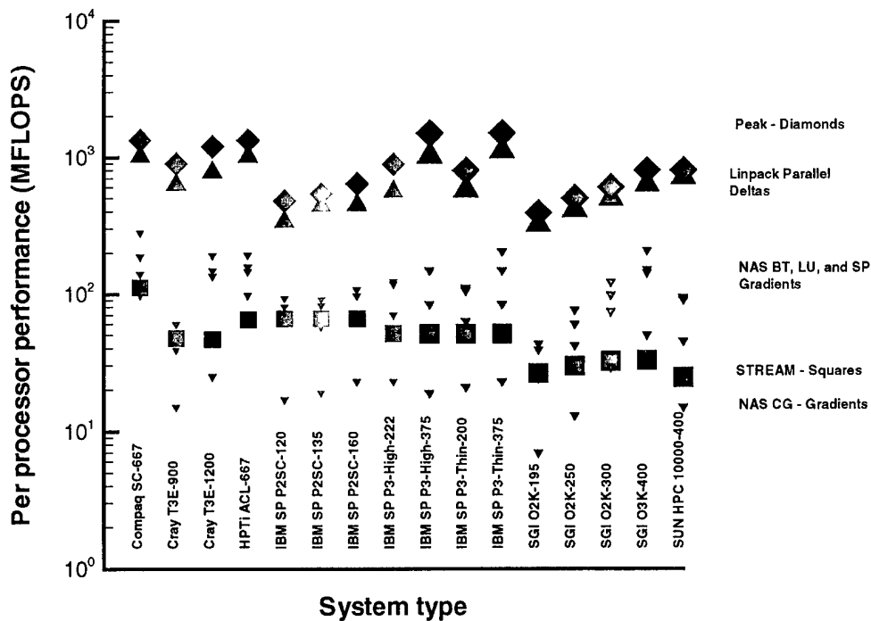
Figure 1. Comparison of commonly used HPC benchmarks (100–200 processors).
