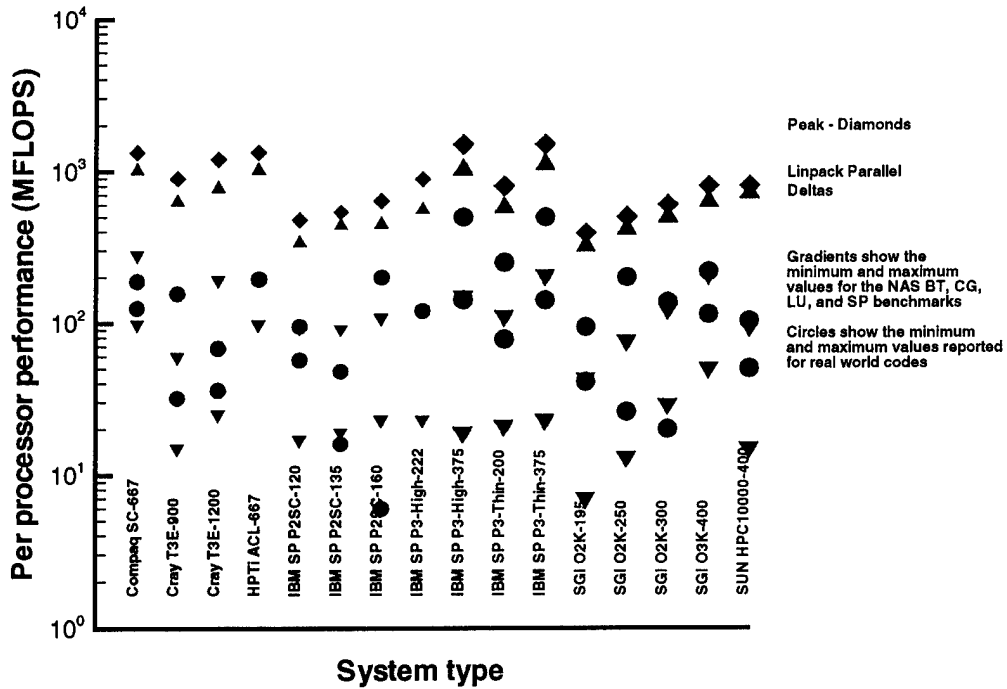
Figure 7. Comparison of commonly used HPC benchmarks to real world codes (<100 processors).
