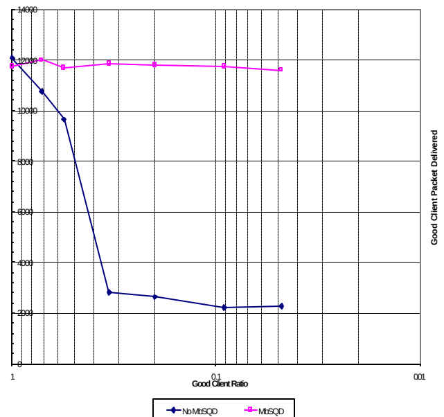
Figure 4-2. MbSQD mitigation against TCP-SYN attacks
