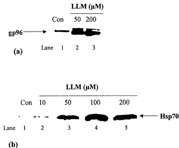
Figure 2. (a), Detection of gp96 in LG-2 cells by Western blot analysis. Cells were either untreated (lane 1) or treated with 50 µM (lane 2) and 200 µM (lane 3) of LLM and lysates (20,000 cells/well) were separated by 12% SDS-PAGE and transferred to PVDF membrane for Western blot analysis. Gp96 was detected using anti-grp94 monoclonal antibody and developed using ECL. (b), Detection of Hsp70 in LG-2 cells by Western blot analysis. Cells were either untreated (lane 1) or treated with 10 µM (lane 2), 50 µM (lane 3), 100 µM (lane 4) and 200 µM (lane 5) of LLM and lysates (20,000 cells/well) were separated by 12% SDS-PAGE and Western blot analysis performed as described above using anti-hsp70 monoclonal antibody.
