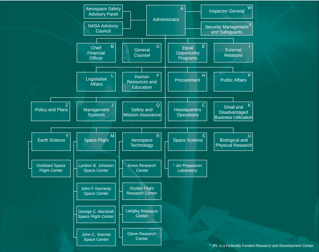
Figure 2: NASA Organization
