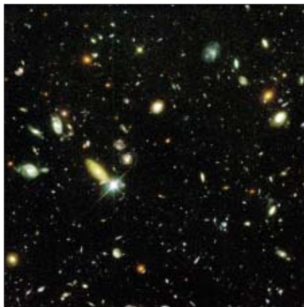
Figure 7: Distant Supernova
