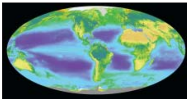
Figure 18: SeaWiFS Data
