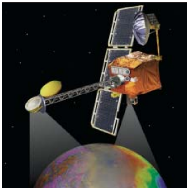
Figure 11: Mars Odyssey
