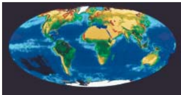
Figure 16: Climate Modeling
