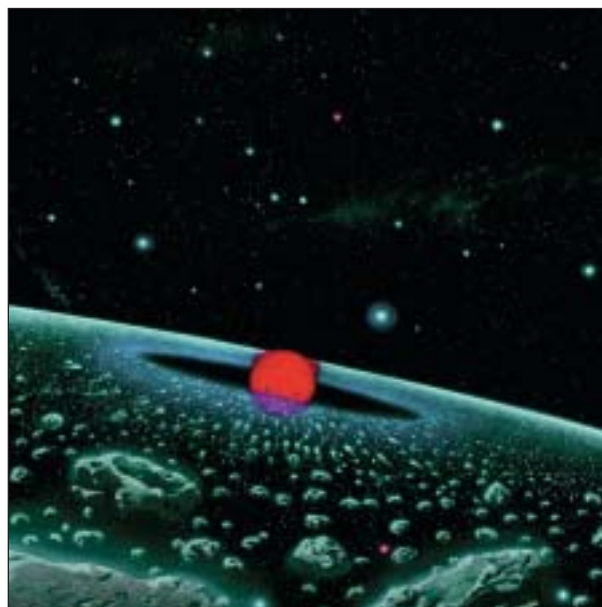
Figure 10: Water-Bearing Worlds Beyond Our Solar System
