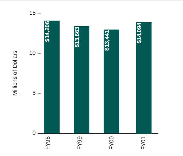
Figure 40: Total Outlays
