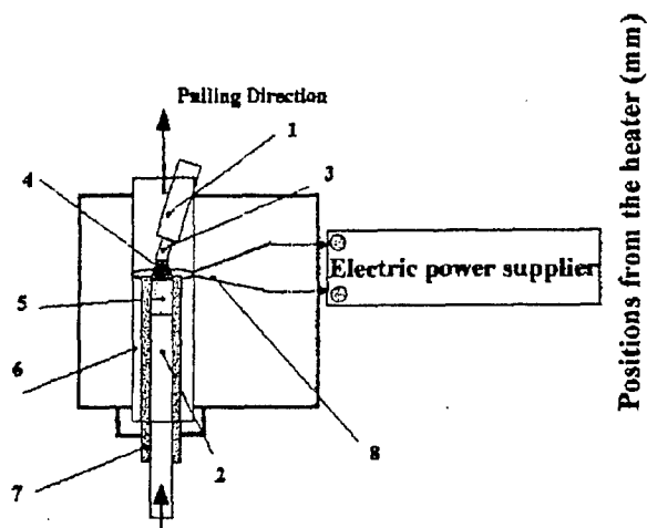
Fig. 1 Schematic diagram of RHHPG. 1: Pulling rod; 2: Pushing rod; 3: Seed crystal; 4: Molten zone; 5: Materials; 6: Inner glass tube; 7: Teflon tube guide; 8: Ring-heater
