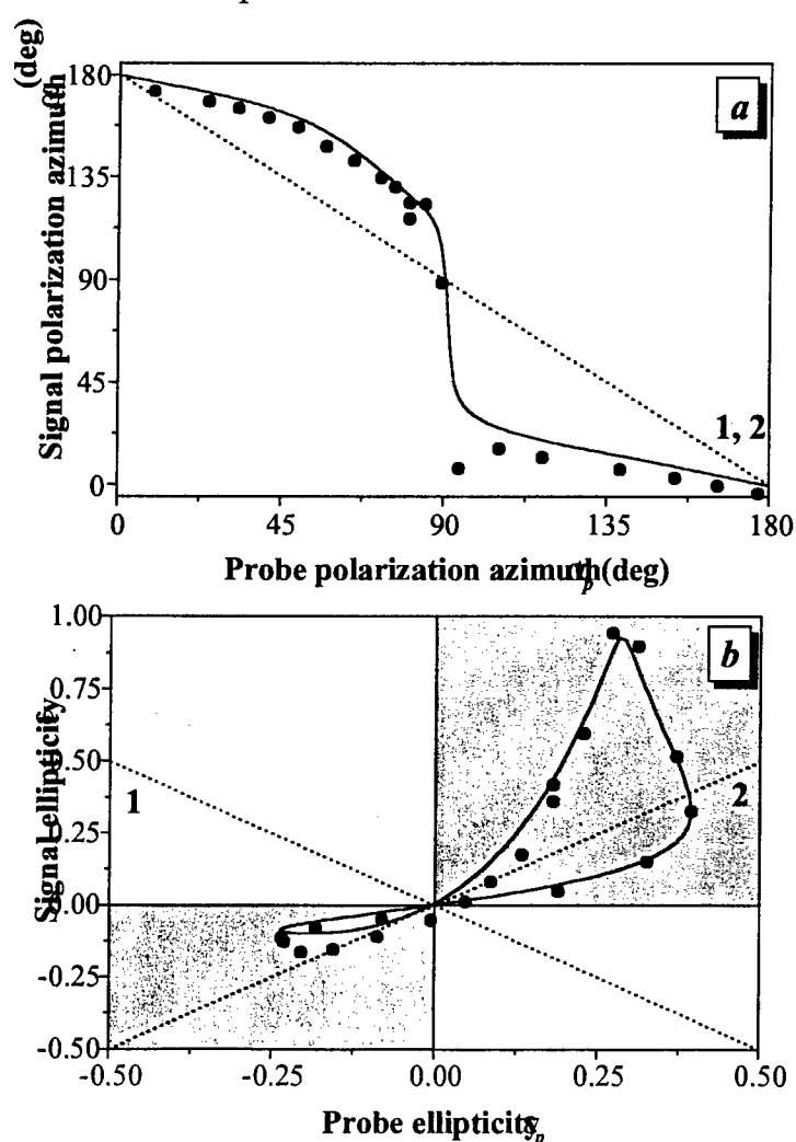
Fig.1. Polarization azimuth (a) and ellipticity (b) of the conjugated (signal) beam versus the same parameters of the probe beam. Circles are experimental data and solid lines are theoretical calculation. Dotted lines 1, 2 show the behaviour of ideal conventional and polarization insensitive phase-conjugate mirrors, respectively.
