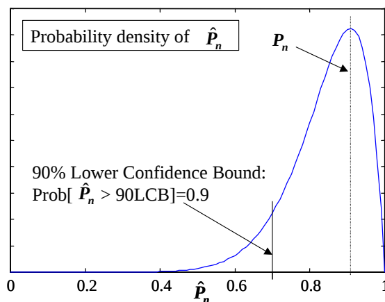
Figure 1 – Estimation Distribution for P_n
