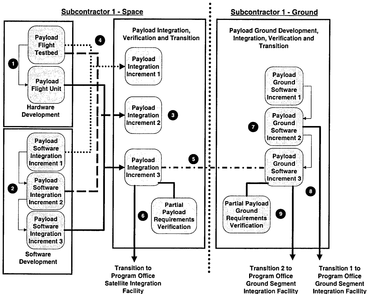
Figure 8. Subcontractor 1 development, integration, verification, and transition relationships.
