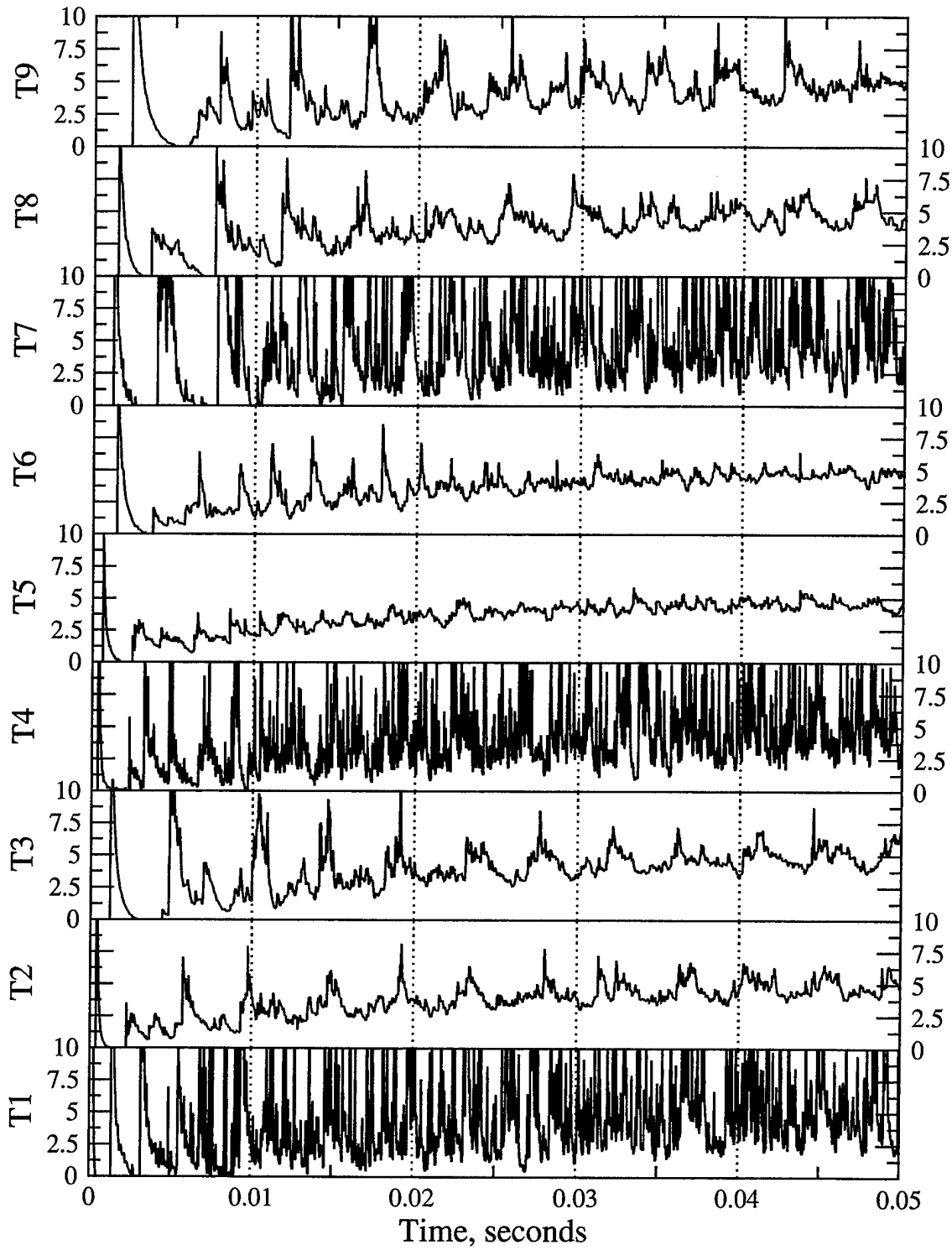
Figure 15: Pressure traces at selected points in the axi-symmetric domain as a function of time. R_b = 11 cm, W_{TNT} = 2.12 kg. Cells = 500. \Delta t = 0.25 \mu s .
