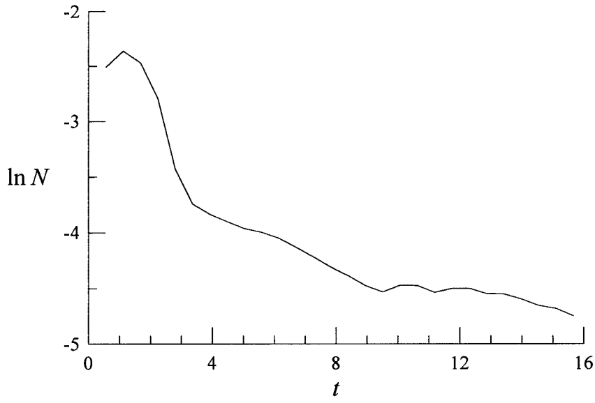
Figure 1.2 Logarithm of the full number of electrons N as a function of time in the case of \gamma_b < \gamma_l .
