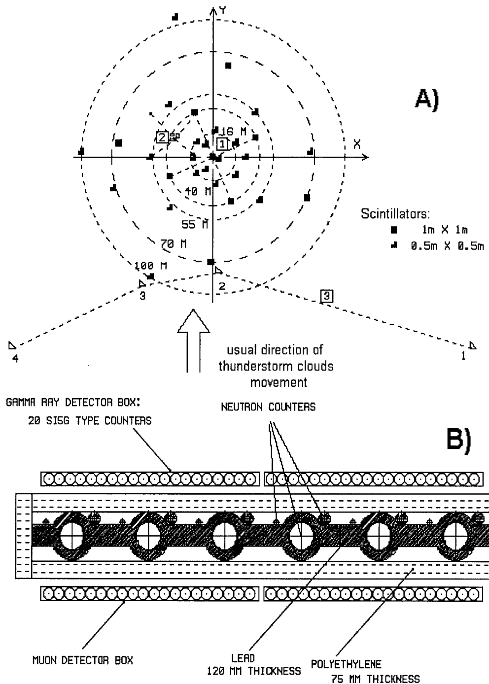
Figure 3.1. Disposition layout of mountain cosmic ray station's detectors (A): 1– the center of shower scintillation system, 2– neutron monitor and high-threshold gamma detectors, 3 – the system of four WS low-threshold gamma- and X-ray detector points, (B): the cross-section of a neutron monitor unit together with high-threshold and muon detectors.
