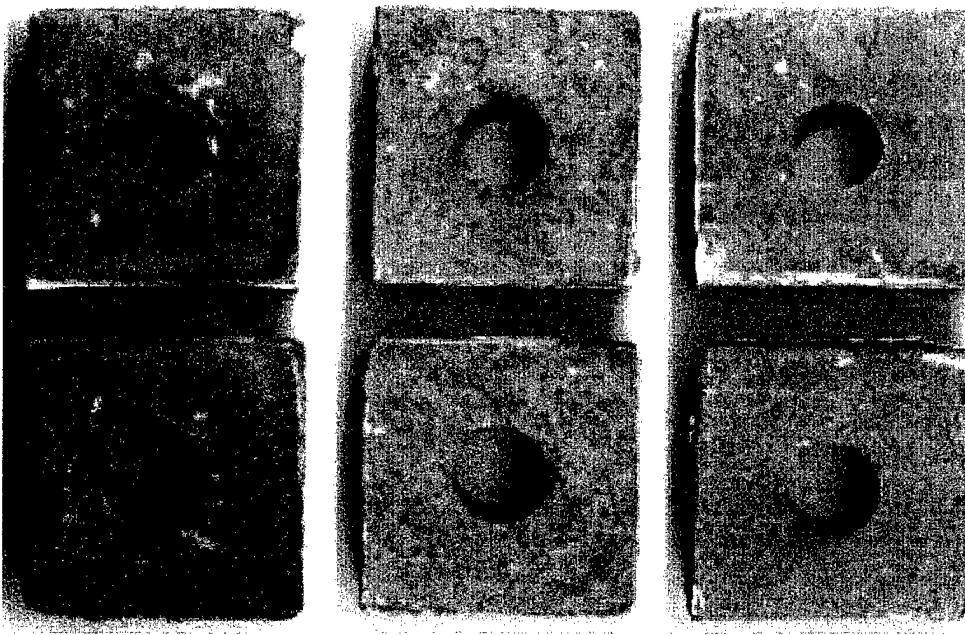
Figure 11. Macrophotos of Ti-steel interfaces after phase II cyclic corrosion exposure.
