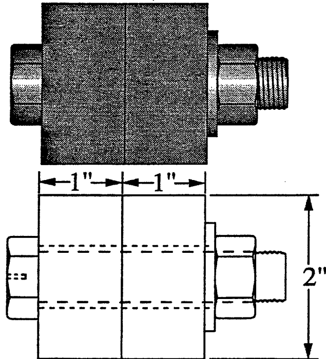
Figure 1. Engineering samples assembled to the "TACOM Joint A Assembly" configuration.
