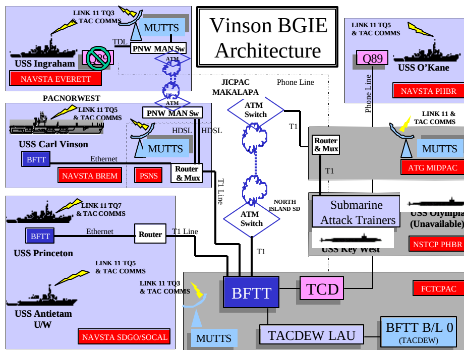
Figure 3. USS CARL VINSON BATTLE Group Training Network
