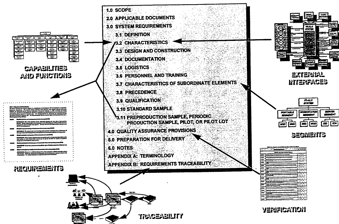
Figure 3-6. SSS Components
