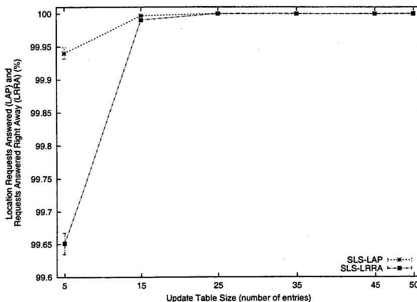
FIG. 4.9. Percent of Location Requests Answered and In Table vs. SLS LP Table Size.
