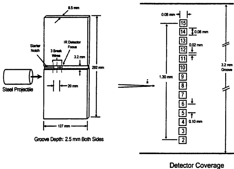
Figure 8. Shear-dominated dynamic fracture experiment configuration also showing infrared detector coverage and painted wires for coarse crack speed measurement. Crack propagates from left to right.
