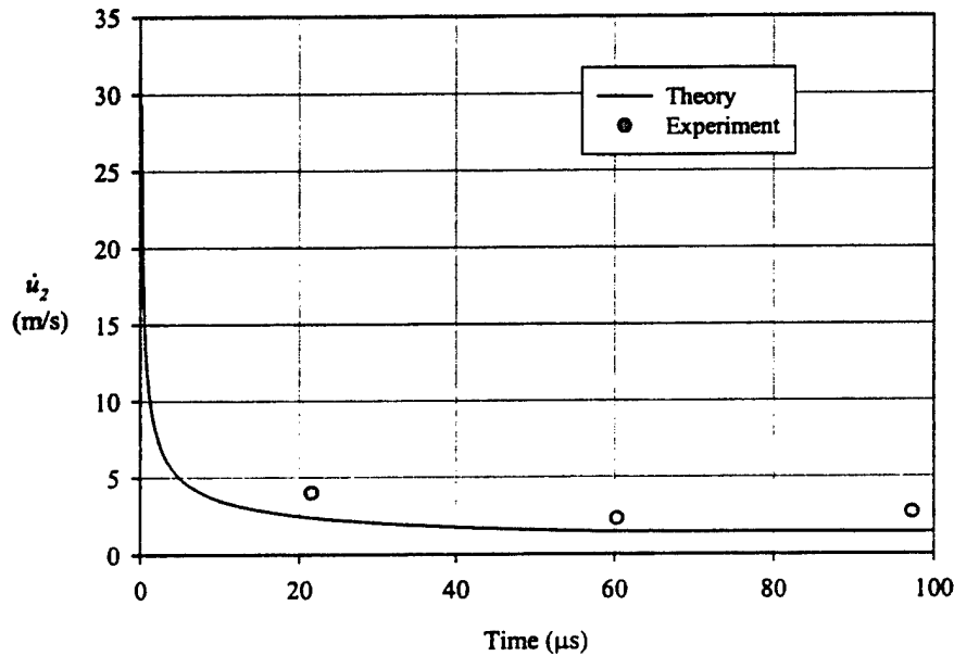
Figure 118. Crack face opening speed for fracture of PMMA with a crack tip speed of 300 m/s. Experimental data derived from temperature measurements are compared to analytical expression from Freund (1990).
