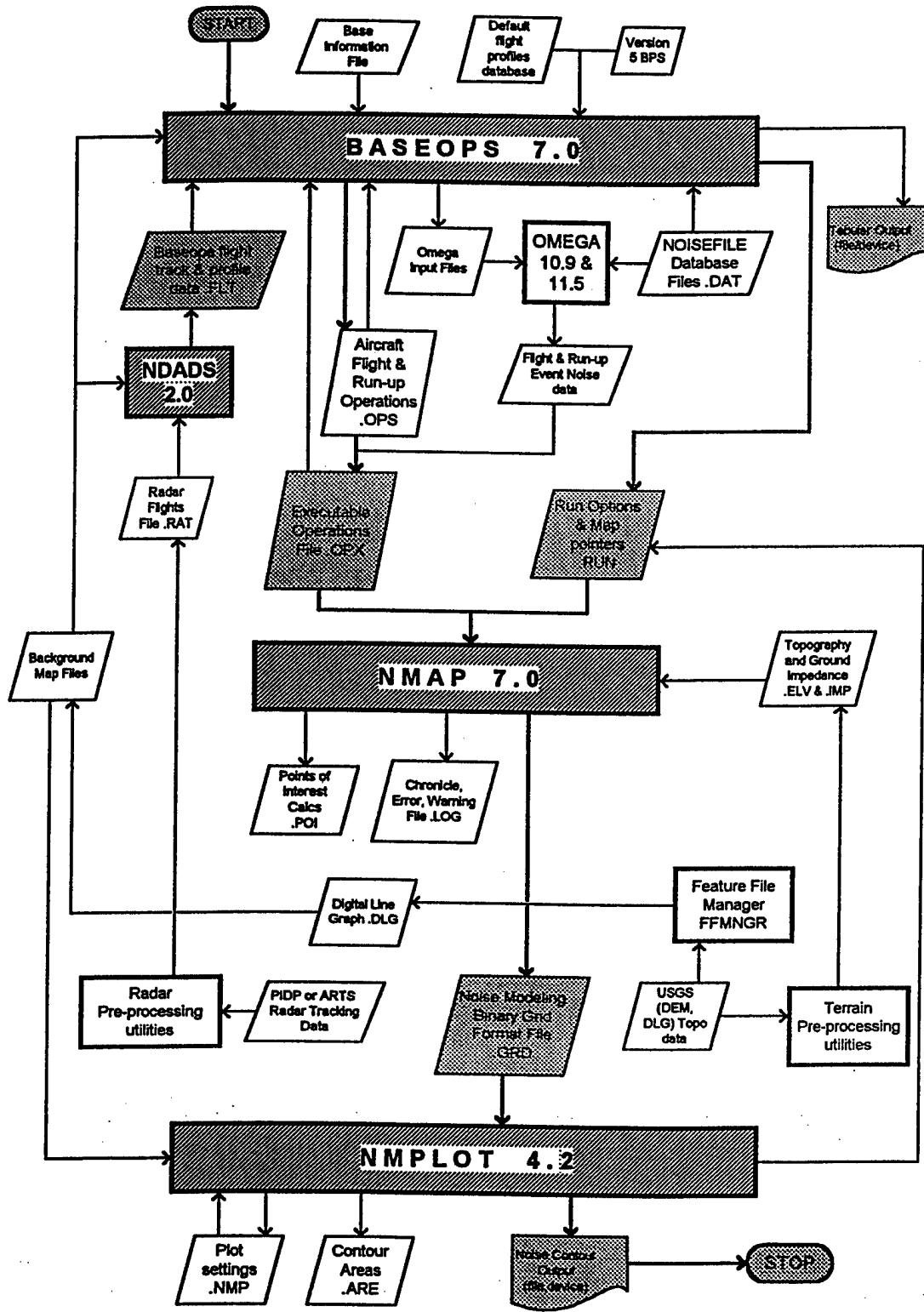
Figure 1-1. NOISEMAP 7.0 Flowchart
