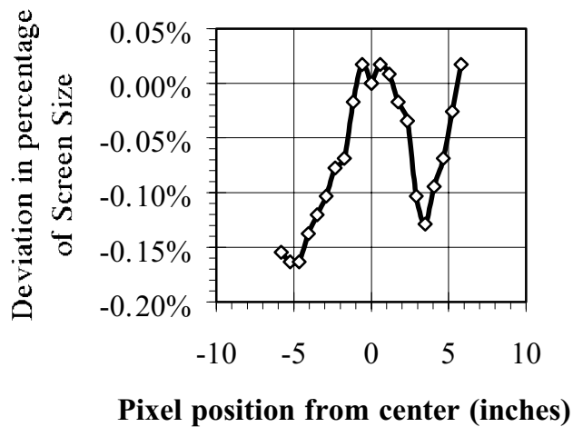
Fig. II.18-4 Vertical linearity characteristic
