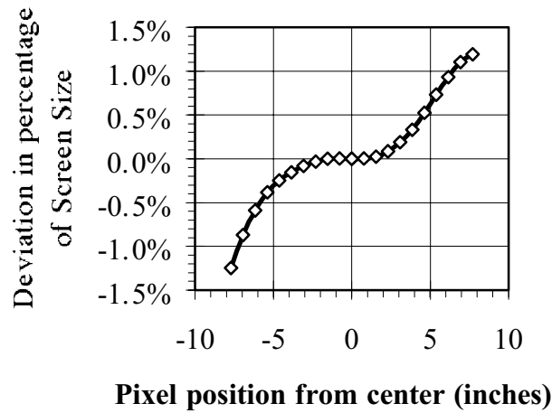
Fig. II.18-3 Horizontal linearity characteristic.
