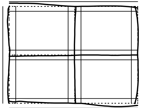
Figure II.15-3 Waviness of Orwin Associates DEX 2102L Monochrome monitor in 1600 x 1200 mode. Departures from straight lines are exaggerated on a 10X scale. Error bars are +/- 0.5% of total screen size.
