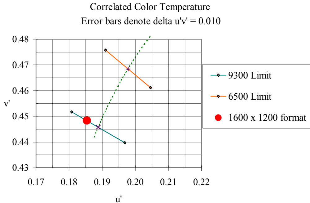
Figure II.5-1. The CCT of the measured white point is within the boundaries required by IEC.
