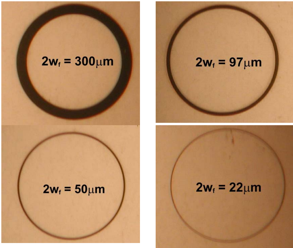
Fig. 1 YBCO rings
