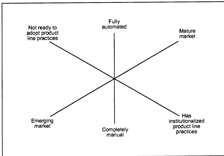
Figure 2: Classification Dimensions
