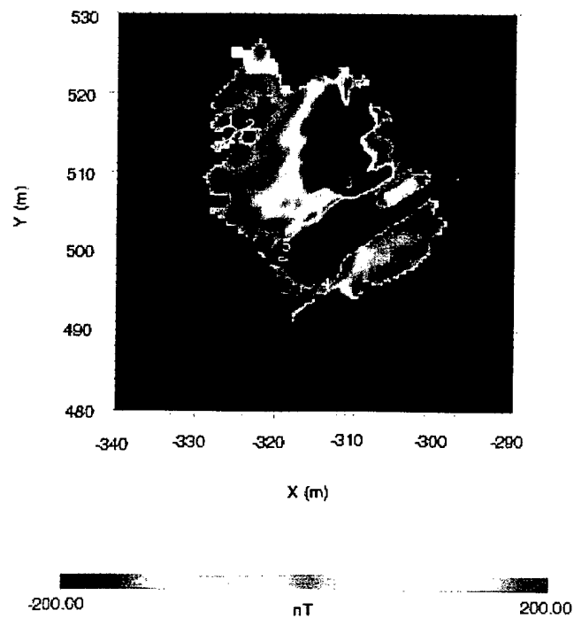
Fig. 16– Magnetic anomaly image map of the north-most area surveyed
