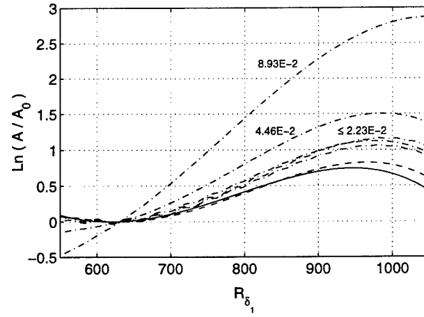
Figure 7: Comparison of growth rates of 2-D TS-waves over a virtual wall at y = 0 for various CFL numbers (— · —), compared with a standard DNS (— — —), and with LST (—). Note: CFL = C\Delta t/\Delta x , and \Delta x is held constant.
