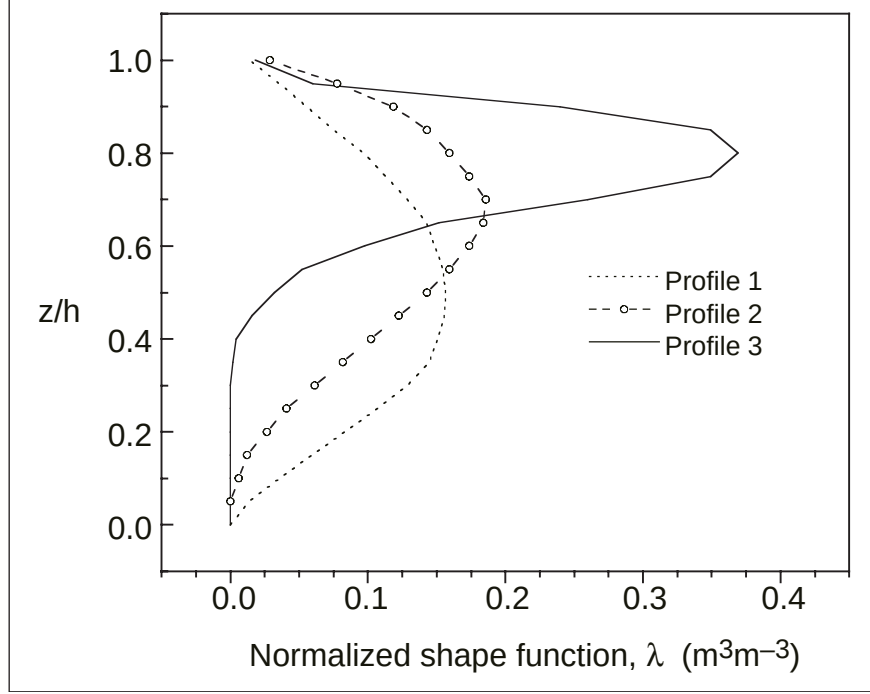
Figure 3. Normalized vertical profiles of leaf area distribution for forest canopies where A(z) = I(z) \cdot LAI (based on Meyers et al. 1998; and Albertson et al. 2001).
