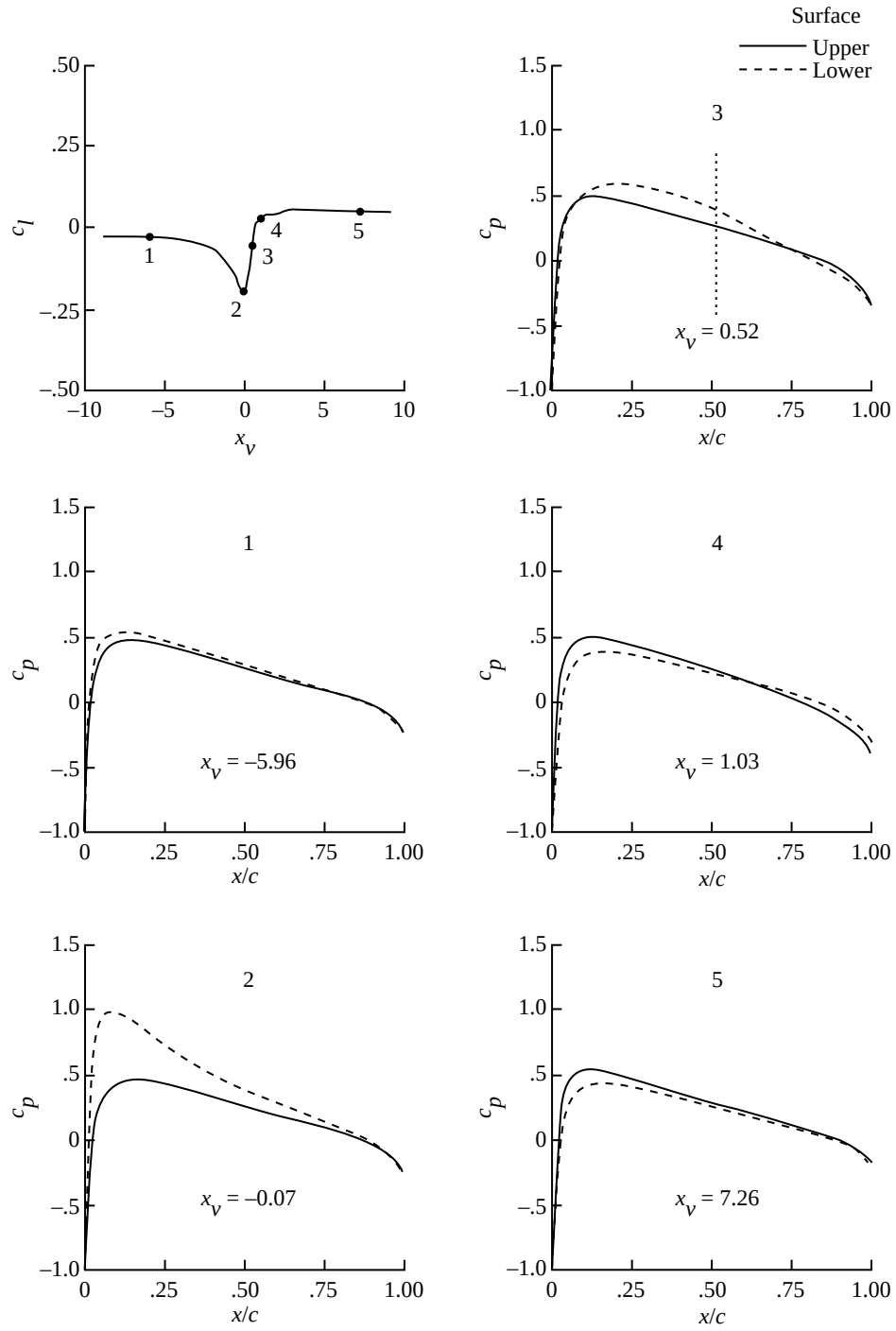
Figure 22. Airfoil surface pressure distribution for typical BVI.
