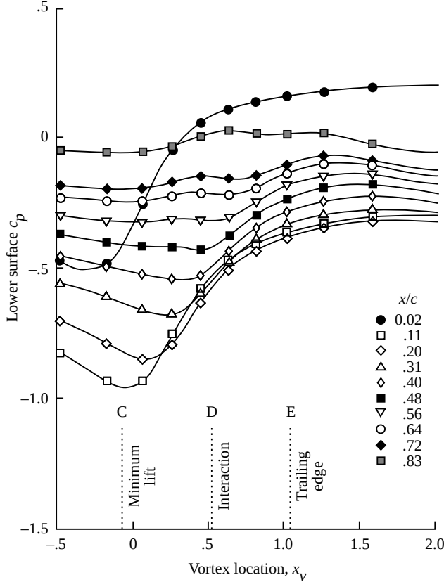
Figure 23. Variation of lower surface pressure coefficient with vortex location for typical BVI.
