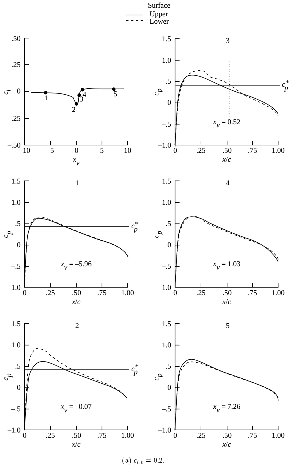
Figure 39. Airfoil pressure distribution at selected vortex locations for several vortex strengths.
