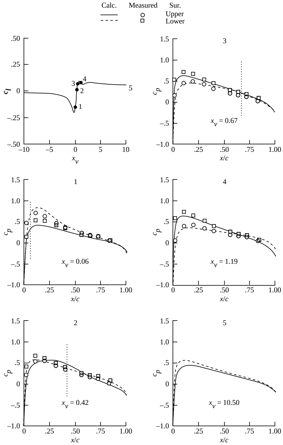
(c) Branch-cut method.
