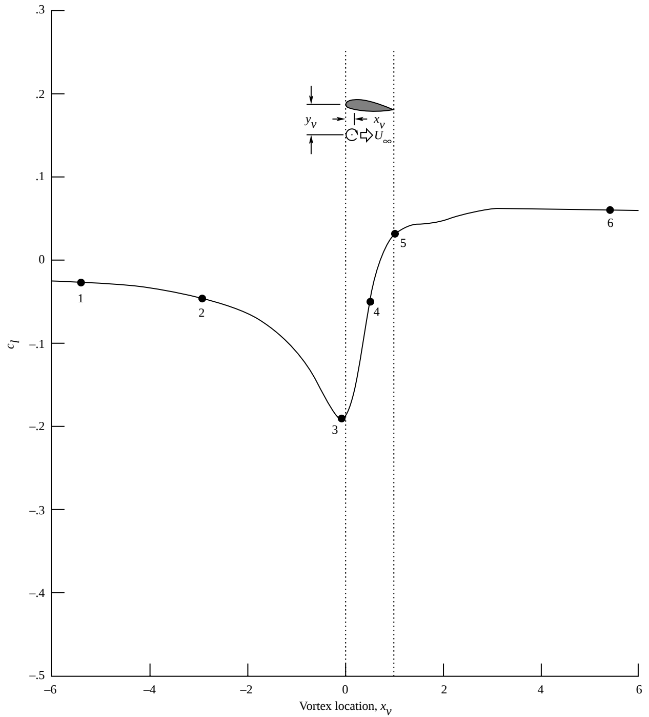
Figure 21. Variation of airfoil lift with vortex location for typical BVI. a = 0.05 ; \alpha = 0^\circ ; M_\infty = 0.60 ; y_v = -0.251 ; c_{l,v} = 0.400 ; NACA 0012 airfoil; fixed path.
