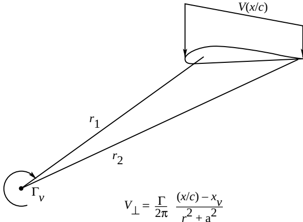
Figure 8. Lifting-surface vortex model.
