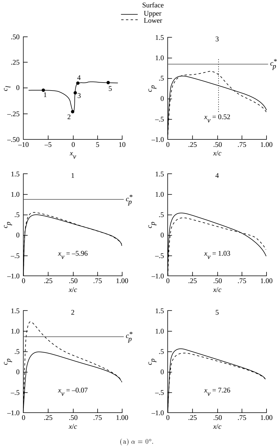
Figure 45. Airfoil pressure distribution at selected vortex locations.
