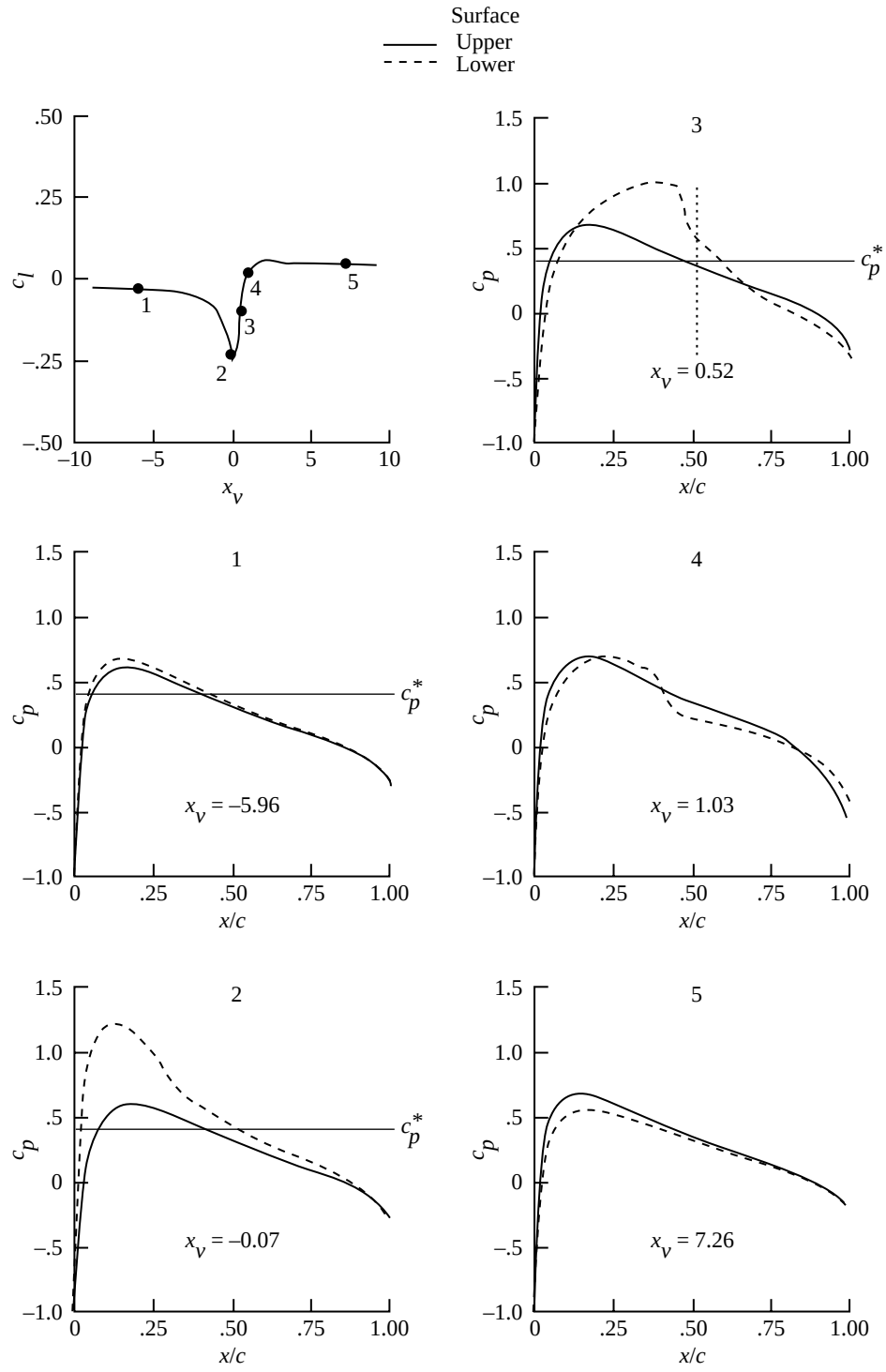
Figure 43. Airfoil pressure distribution at selected vortex locations for several vortex core radii.
