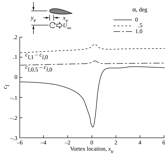
Figure 44. Effect of angle of attack on airfoil lift variation for subcritical flow. a = 0.05 ; M_\infty = 0.60 ; y_v = -0.251 ; c_{l,v} = 0.400 ; NACA 0012 airfoil; fixed path.
