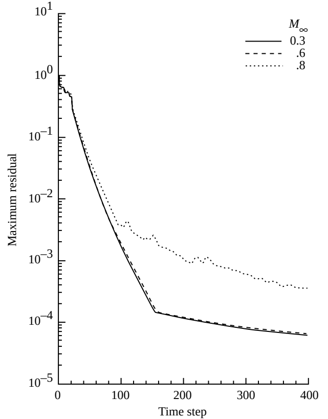
Figure 12. Maximum residual convergence history for NACA 0012 airfoil at several Mach numbers and \alpha = 0^\circ .
