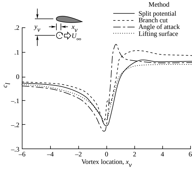
Figure 33. Airfoil lift variation with vortex location for the four vortex models at critical flow. a = 0.15 ; \alpha = 0^\circ ; M_\infty = 0.714 ; y_v = -0.433 ; c_{l,v} = 0.495 ; NACA 0012 airfoil; fixed path.
