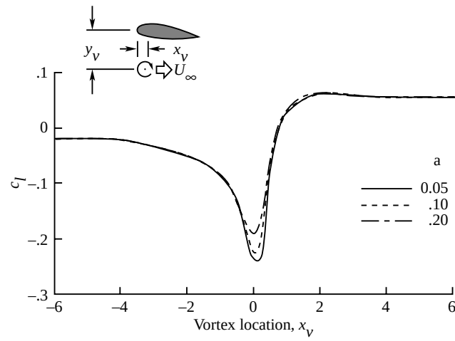
Figure 42. Effect of core size on variation of airfoil lift. \alpha = 0^\circ ; M_\infty = 0.714 ; y_v = -0.251 ; c_{l,v} = 0.400 ; NACA 0012 airfoil; fixed path.
