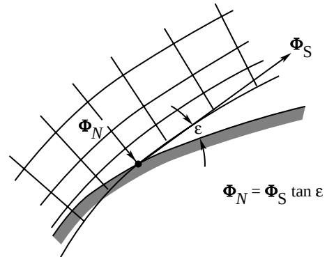
(b) Flow-through condition on coordinate which approximates body (generalization of small-disturbance boundary condition).
