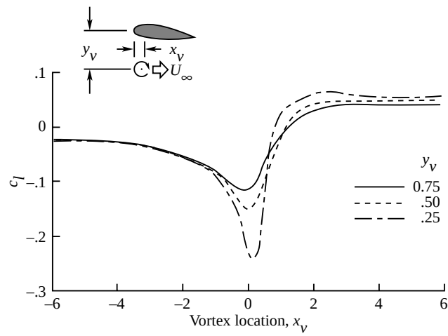
Figure 40. Effect of vertical miss distance on variation of airfoil lift coefficient. a = 0.05 ; \alpha = 0^\circ ; M_\infty = 0.714 ; c_{l,v} = 0.400 ; NACA 0012 airfoil; fixed path.
