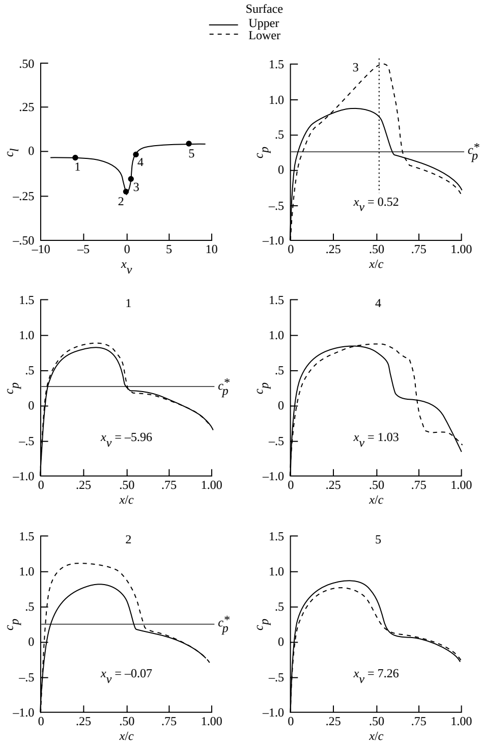
Figure 47. Airfoil pressure distribution at selected vortex locations.
