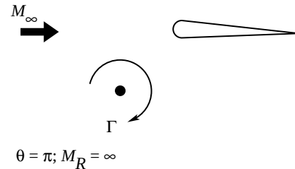
Figure 3. High-speed interaction between rotor and vortex.
