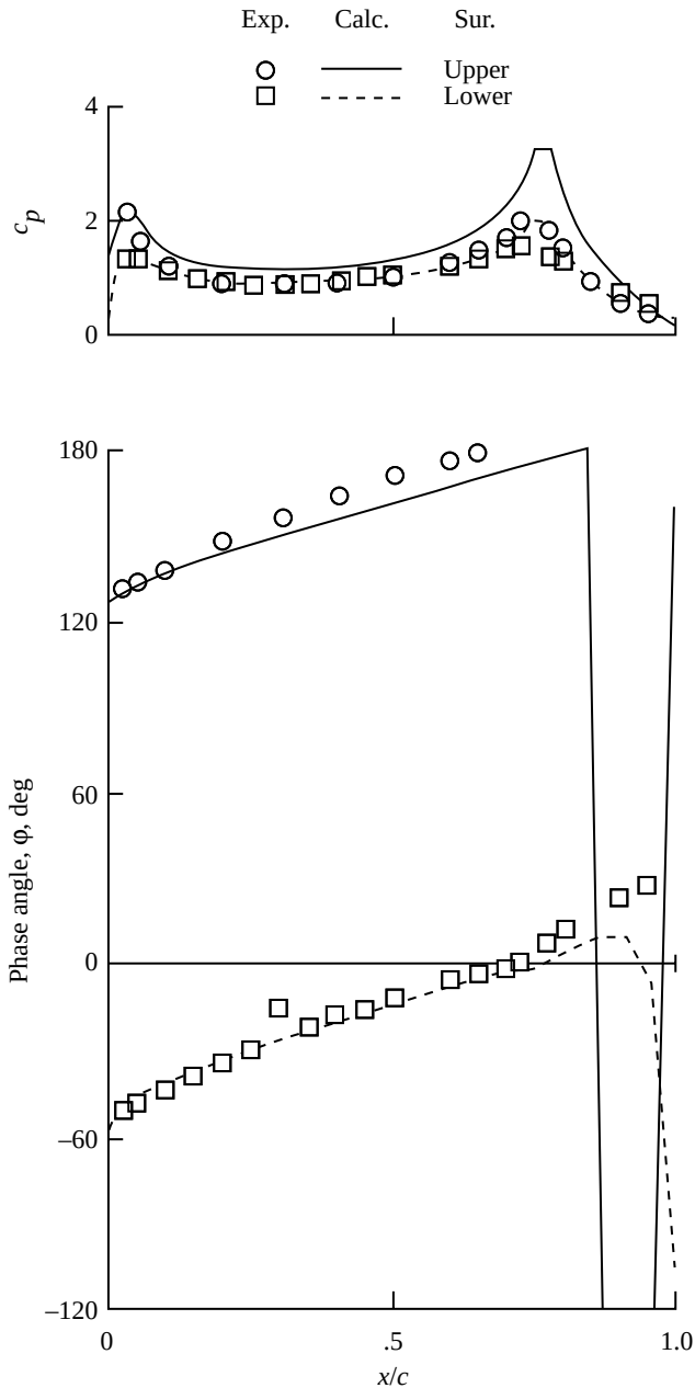
Figure 20. Pressure coefficients for Aerospatiale RA16SC1 airfoil with oscillating 25-percent flap. M_\infty = 0.30 ; \alpha = 0^\circ .
