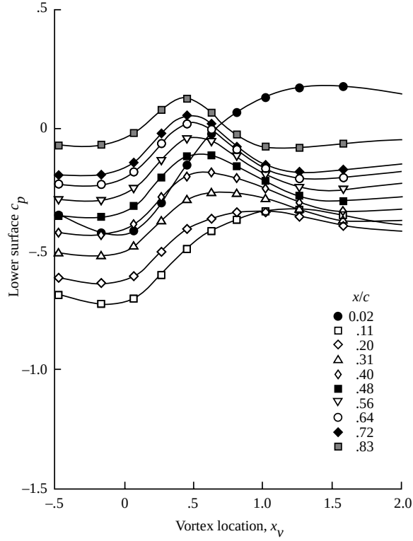
(a) Angle-of-attack method.
