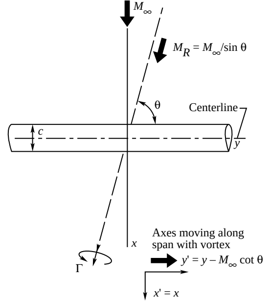
Figure 1. Interaction of infinite aspect ratio blade with infinite line vortex.
