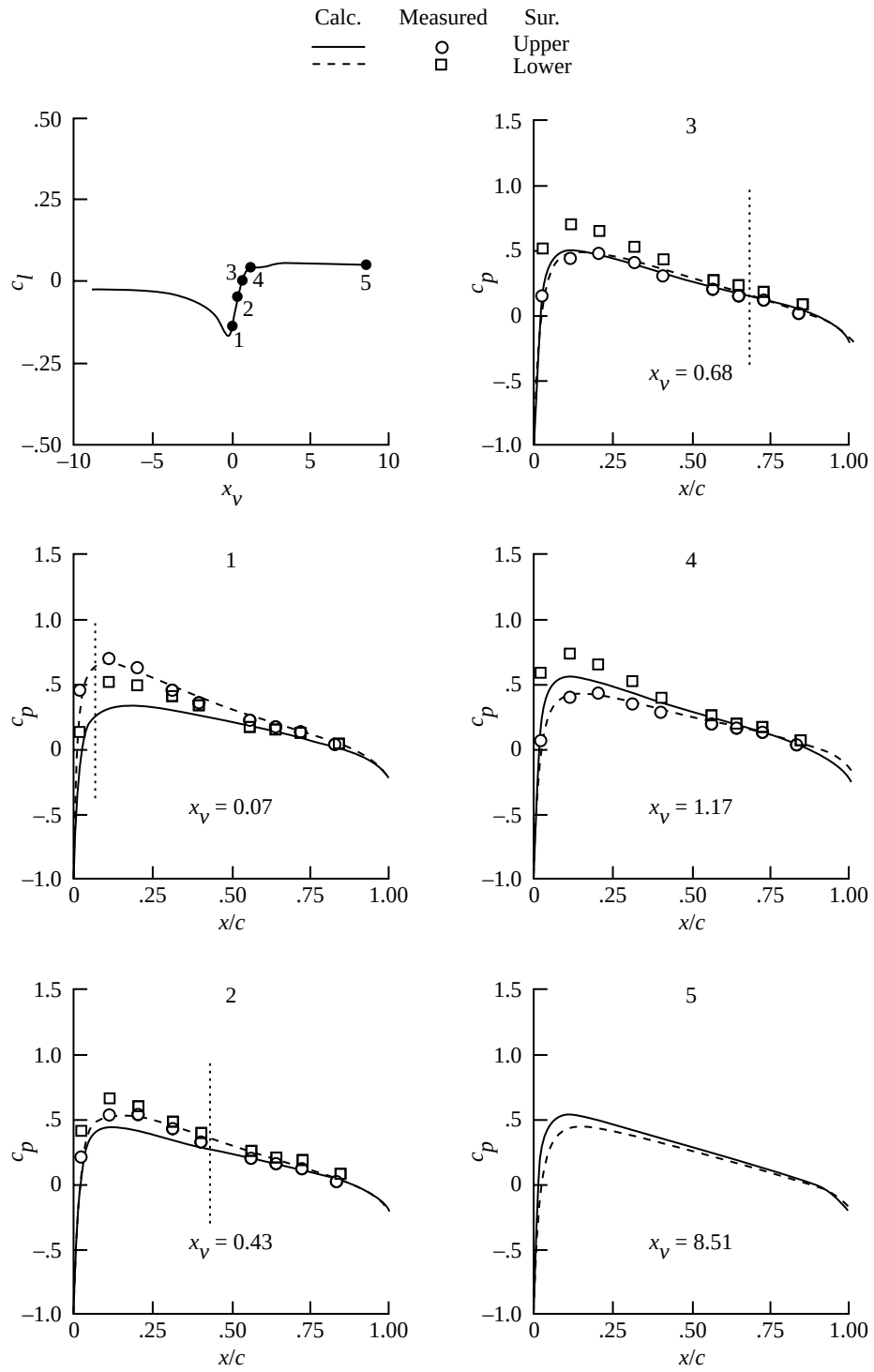
(b) Lifting-surface method.
