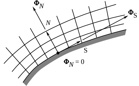
(a) Flow tangency on body conforming coordinate.
