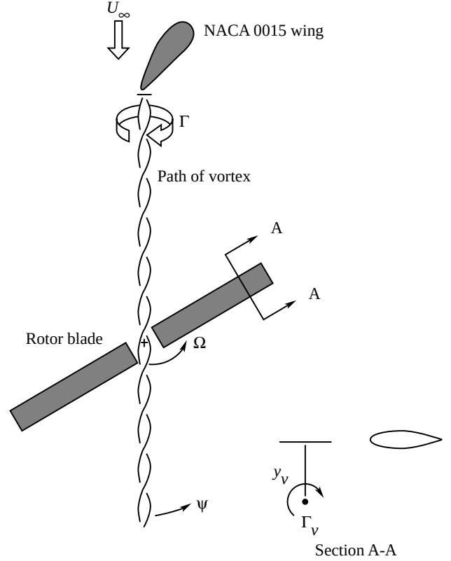
Figure 29. Experimental measurement of blade-vortex interaction.
