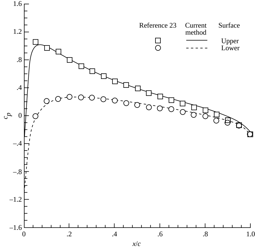
Figure 14. Pressure coefficients for NACA 0012 airfoil at M_\infty = 0.63 and \alpha = 2^\circ .
