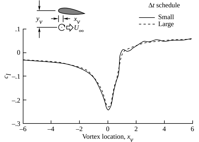
(b) Supercritical flow; a = 0.05 ; \alpha = 0^\circ ; M_\infty = 0.80 ; y_v = -0.251 ; c_{l,v} = 0.40 ; NACA 0012 airfoil; fixed path.
