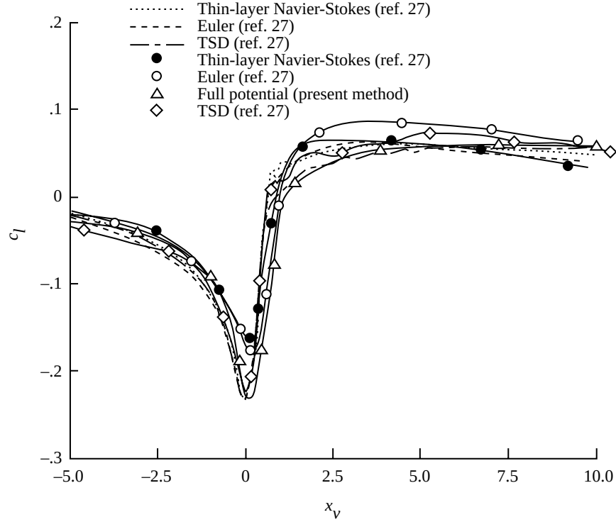
(b) Supercritical flow. M_\infty = 0.80 .
