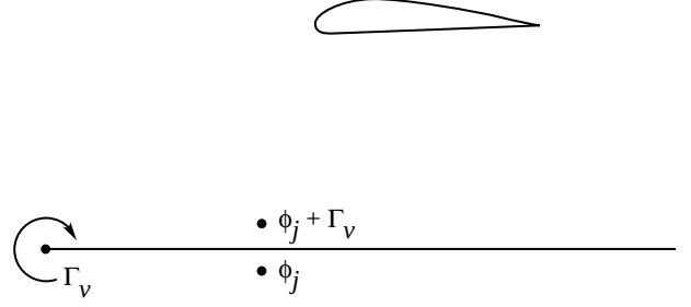
Figure 9. Branch-cut vortex model.
