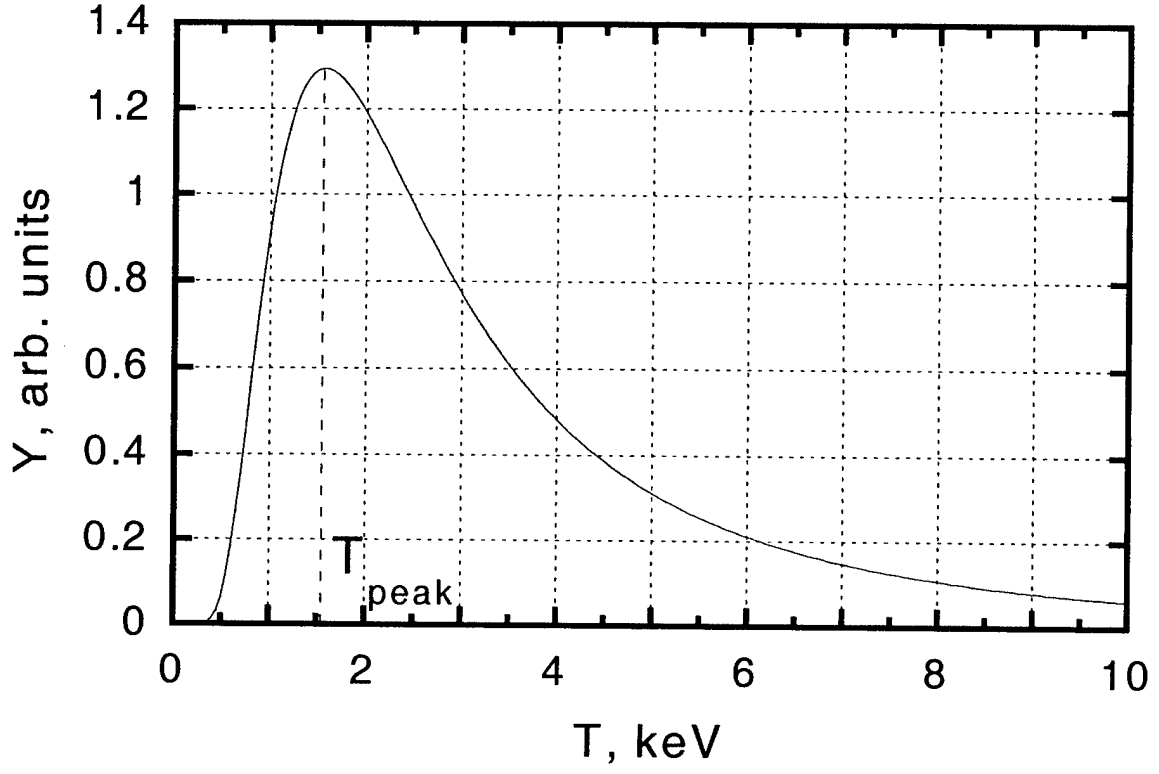
Figure 2. Yield function (13) calculated for aluminum ( Z = 13 ) and E_0 = 7 keV, and shown in arbitrary units. The function peaks at T = T_{\text{peak}} = 1.57 keV.
