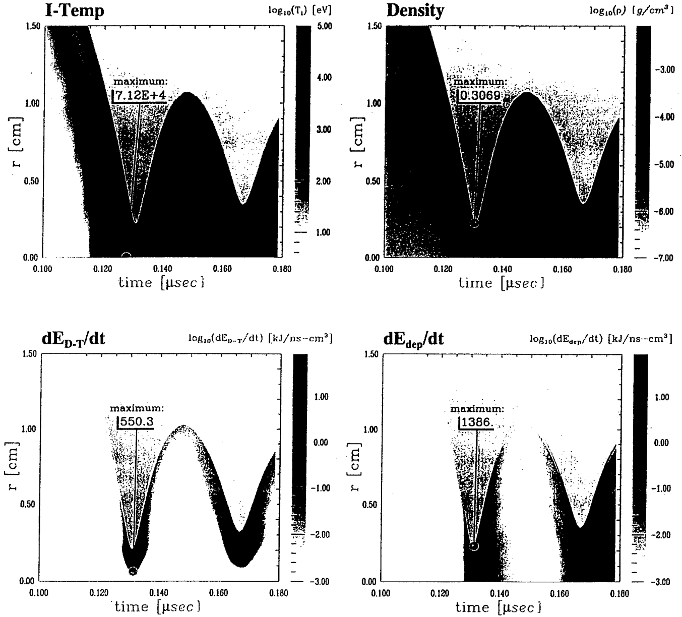
Fig. 3: Implosion history of 40 MA Au/CH/DT/CH Shell.
