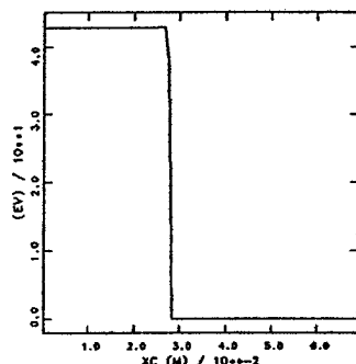
Milne BC profile is "hotter", but breaks at the point where the standard profile abruptly changes the slope.
