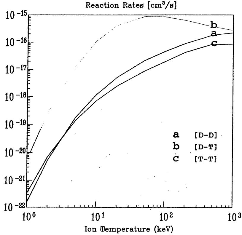
Figure 5: Nuclear fusion reaction rates for deuterium and tritium
