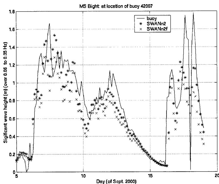
Fig. 23— Wave height comparison between cases with and without bottom friction
