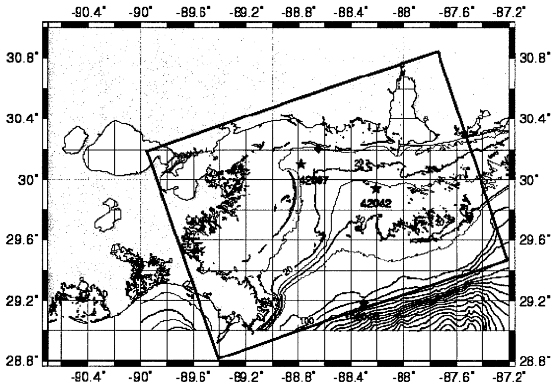
Fig. 1 — NGLI depths in meters, locations of NDBC buoys (stars), SeaBird pressure gauge (square), and Neptune buoy (triangle)
