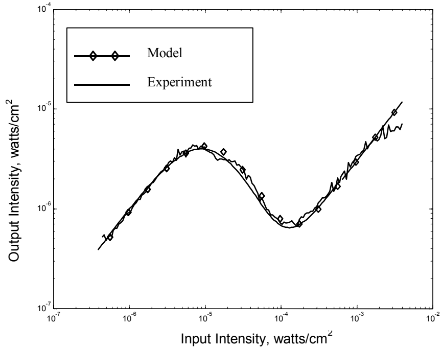
Figure 5-21 EOPL transmission plot and modified model.
