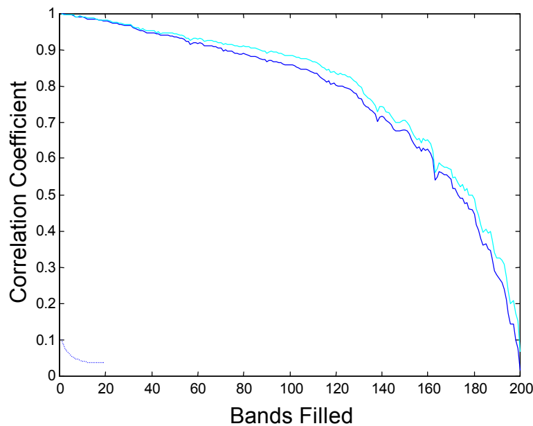
Figure 3-4 Correlation versus spectrum bands filled by high intensity components.
