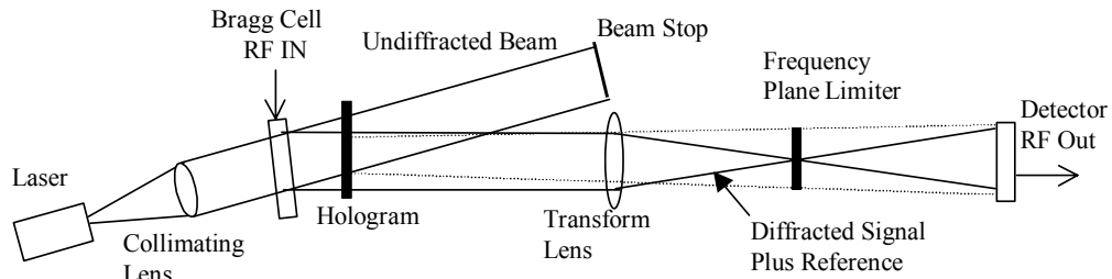
Figure 3-14 Collinear architecture for acousto-optic RF signal excision.
