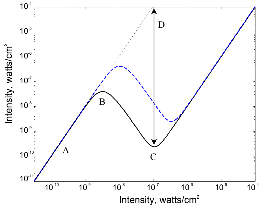
Figure 4-7 Amplitude transmission plot for EOPL using simple model. Dashed line shows effect of control-illumination bias.
