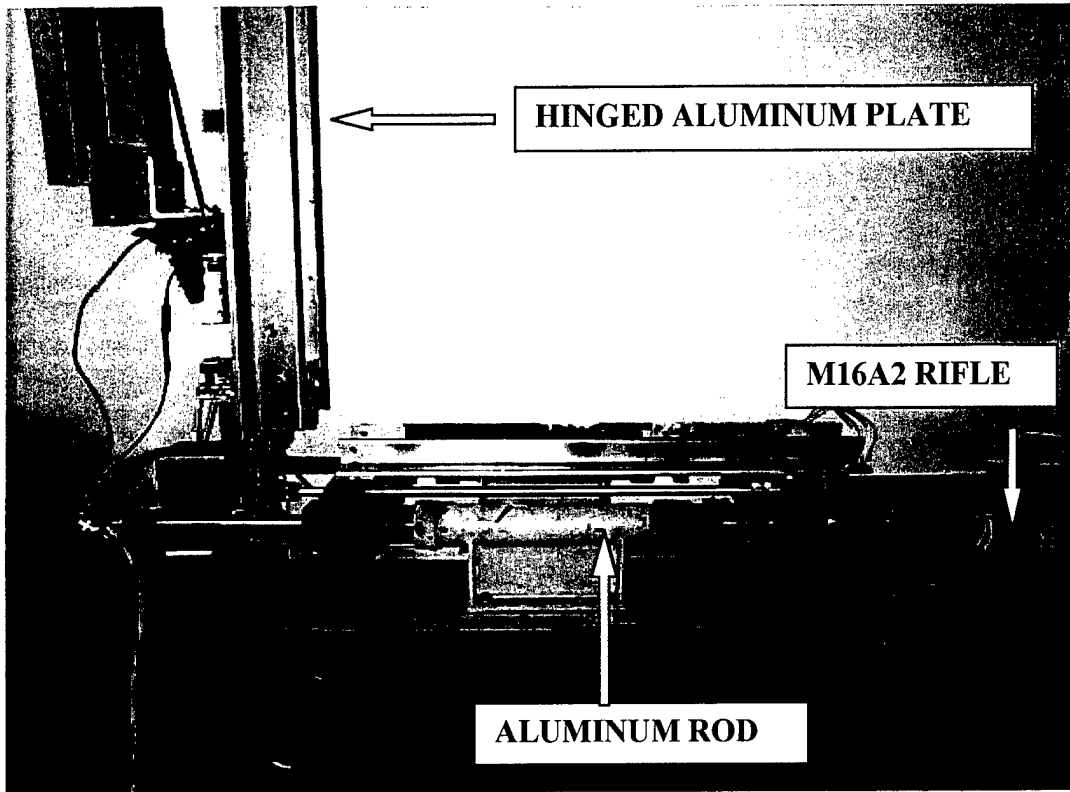
Figure 1. Experimental firing fixture.
