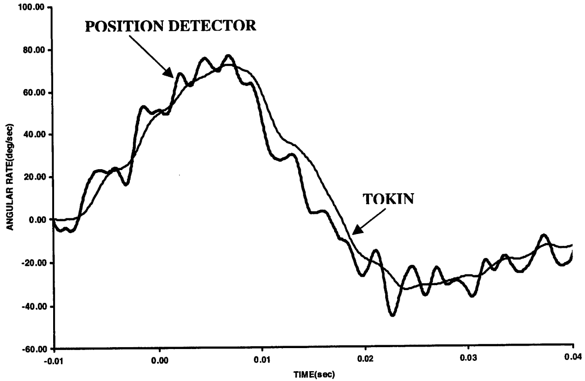
Figure 9. Angular rate versus time for tokin angular rate sensor during firing experiments.
