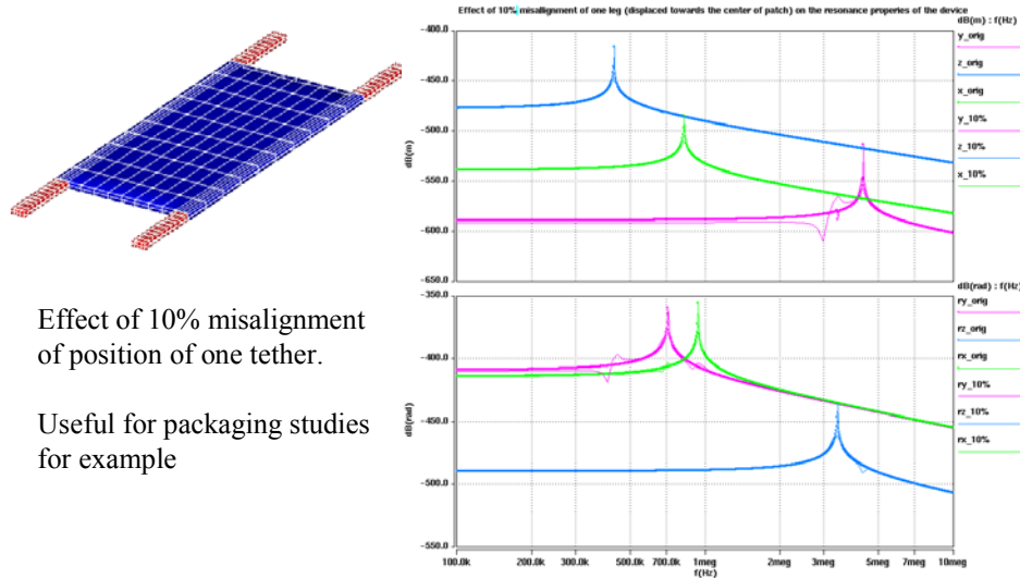
Figure 16: SPCMems - misalignment of tether anchor. Very useful for exploring packaging effects.
