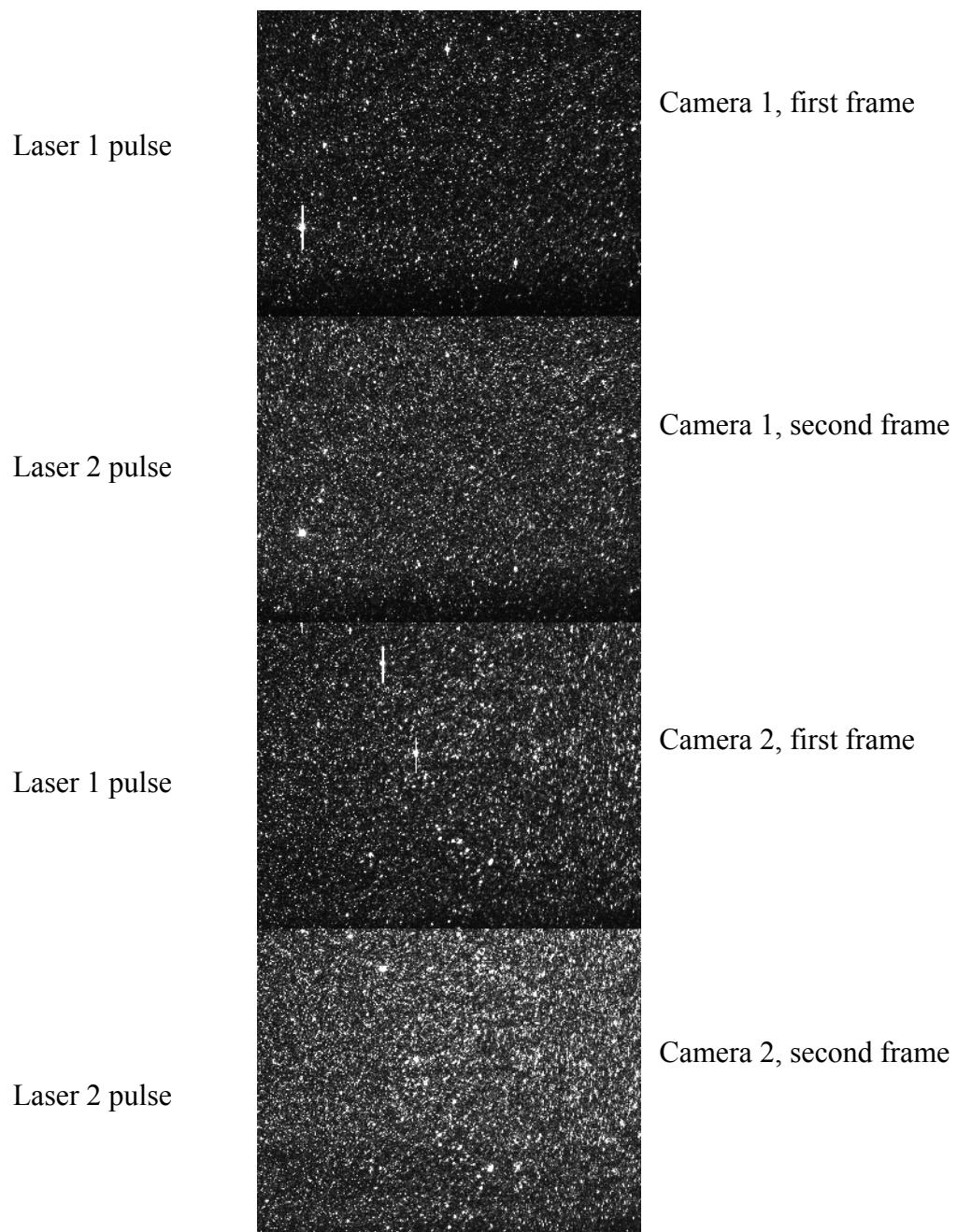
Figure 5.35. Typical PIV images taken with stereo PIV sytem using double frame double exposure mode.
