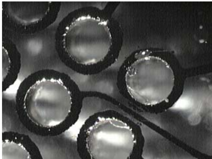
Figure 5.6. Closeup views of MEKA-0 electrokinetic microactuator array prior to polymer filling, showing (a,b) top-surface ring electrodes for each actuator, (c) bottom-surface common electrode, and (d) channel edge chipping resulting from mechanical drilling in glass wafer.
