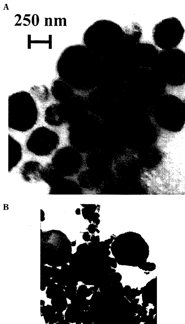
Figure 3. Transmission electron micrographs of a network structure resulting from the hybridization of a 50 \mu\text{g/mL} target sample before (A) and after (B) the 8 min silver enhancement. Hybridization time was 20 min. Micrographs were taken with a Hitachi H7000 instrument, using an accelerating voltage of 75 kV.
