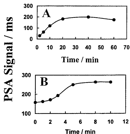
Figure 6. Effect of hybridization time (A) and gold oxidation time (B). Target concentration, 20 \mu\text{g}/\text{mL} ; gold oxidation time (A), 3 min; hybridization time (B), 20 min; amount of magnetic beads, 70 \mu\text{g} ; amount of the 5-nm streptavidin-coated gold particles, 3.8 \times 10^{10} . Other conditions, as in Figure 2.
