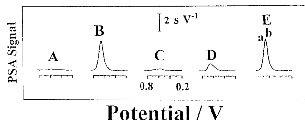
Figure 7. PSA hybridization response to 0 \mu\text{g}/\text{mL} target (A); 25 \mu\text{g}/\text{mL} target (B and E,a); 100 \mu\text{g}/\text{mL} noncomplementary strand (C); 40 \mu\text{g}/\text{mL} three-base mismatched strand (D); a mixture of 25 \mu\text{g}/\text{mL} target and 100 \mu\text{g}/\text{mL} noncomplementary strands (E,b). Hybridization time, 20 min; amount of magnetic beads, 90 \mu\text{g} ; amount of 5-nm streptavidin-coated gold particles, 7.6 \times 10^{10} . Other conditions, as in Figure 2.
