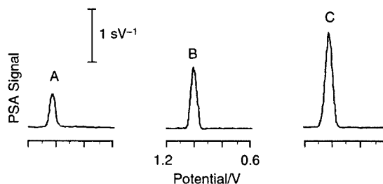
Fig. 7 The potentiometric stripping response for different concentrations of a 57 bp-long target: (A) 0; (B) 5; and (C) 10\ \text{mg l}^{-1} . Beads amount, 10 \mu\text{g} ; probe (guanine-containing) concentration, 200\ \text{mg l}^{-1} ; hybridization time, 5 min. Other conditions, as in Fig. 2.
