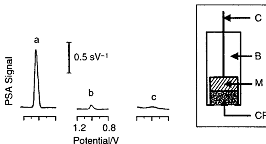
Fig. 8 The stripping hybridization response of the magnetic-carbon paste electrode (MCPE) to 5\ \text{mg l}^{-1} of the 19 bp-long target (a), 50\ \text{mg l}^{-1} three-base mismatched oligomer (b) and 150\ \text{mg l}^{-1} non-complementary oligomer (c). Beads amount, 50\ \mu\text{g} ; probe concentration, 200\ \text{mg l}^{-1} ; hybridization time, 10 min; stripping current, +5.0\ \mu\text{A} . The MCPE is shown in the inset (M, magnet; CP, carbon paste; B, body; C, contact).
