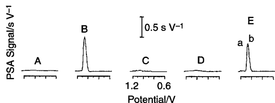
Fig. 2 Chronopotentiometric stripping hybridization response to: (A) the blank solution; (B) 20 \text{ mg l}^{-1} ( \mu\text{g ml}^{-1} ) 19 bp long target T; (C) 100 \text{ mg l}^{-1} non-complementary (NC) oligomer; (D) 50 \text{ mg l}^{-1} three-base mismatched oligomer; (E, a) a mixture of 15 \text{ mg l}^{-1} T and 150 \text{ mg l}^{-1} NC; 15 \text{ mg l}^{-1} T; (E, b) amount of beads, 100 \mu\text{g} ; probe concentration, 200 \text{ mg l}^{-1} ; hybridization time, 5 min; stripping current, +5.0 \mu\text{A} ; accumulation potential +0.5 V for 1 min. Graphite (pencil) electrode pretreated at +1.4 V for 1 min.
