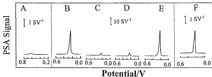
Figure 2. Chronopotentiometric stripping response for DNA detected by monitoring the gold nanoparticle tag (A) and the silver enhancer tag (B–F): 200 ng/mL target (A); 200 ng/mL target (B); 10 \mu\text{g/mL} noncomplementary strand (C); 600 ng/mL three-base mismatched strand (D); a mixture of 200 ng/mL target and 10 \mu\text{g/mL} noncomplementary strand (E); 20 ng/mL target (F). Gold assay conditions: (A) deposition, 1 min at -0.8 V; stripping current, +3.0 \mu\text{A} . Silver assay conditions (B–F): deposition, 1 min at -0.5 V; stripping current, +3.0 \mu\text{A} . Hybridization time, 20 min; amount of the magnetic beads (Bangs Laboratories), 50 \mu\text{g} ; amount of 20 nm streptavidin-coated gold particles (Energy Beam Science), 5 \mu\text{L} . Silver Enhancer Solution (Sigma, equal volumes of solutions A and B), 30 \mu\text{L} each; 60 \mu\text{L} 2.5% sodium thiosulfate pentahydrate. Oligonucleotides (with 5' biotin modification) were acquired from Sigma-Genosys Ltd. and had the following sequences: biotin-5'GAT TTT CTT CCT TTT GTT C (immobilized probe, E908X-WT/P); biotin-5'GAA CAA AAG GAA GAA AAT C (target, E908X-WT); biotin-5'GGT CAG GTG GGG GGT ACG CCA GG (noncomplementary strand, E908X); biotin-5' CAA CAA AAG CAA CAA AAT C (mismatched strand, E908X-WT/3bm). Chronopotentiometric measurements were performed with a TraceLab stripping unit PSU20 (Radiometer). DNA assays were carried out using the MCB 1200 Biomagnetic Processing Platform (Dexter Corp. Magnetic Technologies, Fremont, CA).
