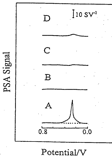
Figure 4. Chronopotentiometric hybridization signals for (A) the 200 \text{ ng mL}^{-1} BRCA1 DNA target (with and without an external magnet; solid and dotted lines, respectively), (B) 20 \text{ } \mu\text{g mL}^{-1} non-complementary strand, (C) 600 \text{ ng mL}^{-1} 3-base mismatched oligomer, and (D) 200 \text{ ng mL}^{-1} one-point mutated oligonucleotide. Hybridization time, 20 min; silver enhancement time, 10 min (From ref. 5.)
