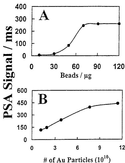
Figure 4. Effect of the amount of magnetic beads (A) and amount of streptavidin-coated gold particles (B) upon the hybridization response to the 20 \mu\text{g}/\text{mL} target. Probe concentration, 200 \mu\text{g}/\text{mL} ; amount of the 5-nm streptavidin-coated gold particles (A), 3.8 \times 10^{10} ; amount of the magnetic beads (B), 90 \mu\text{g} ; probe concentration, 200 \mu\text{g}/\text{mL} ; hybridization time, 20 min. Other conditions, as in Figure 2.
