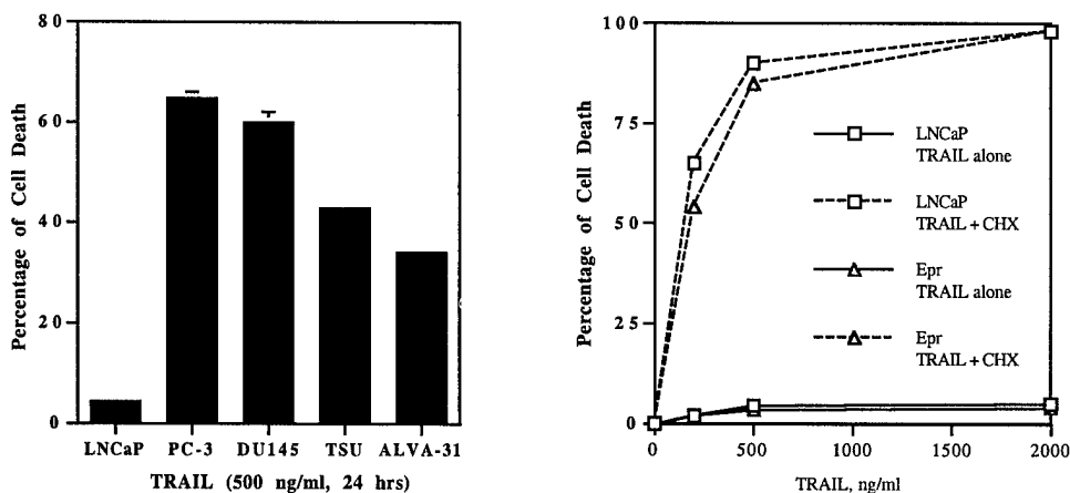
Figure 1. TRAIL sensitivity of normal prostate epithelial cells and various prostate cancer cells. A. TRAIL sensitivity of 5 PC cells. PC cells were treated with purified His-tagged TRAIL for 24 hours, and the percentage of cell death was measured with MTT assay. B. The effect of cycloheximide (CHX)
