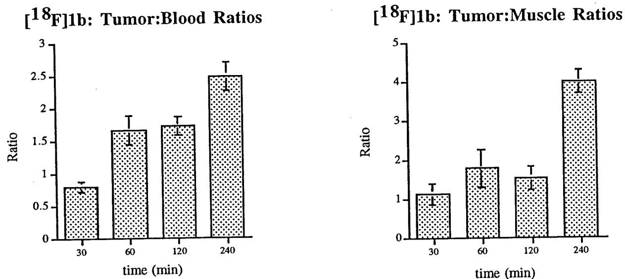
Figure 1. Tumor: blood and tumor: muscle ratios of [ 18 F]1b in tumor bearing mice.
