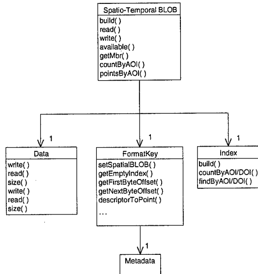
Figure 1. An object decomposition of the Spatio-Temporal BLOB
