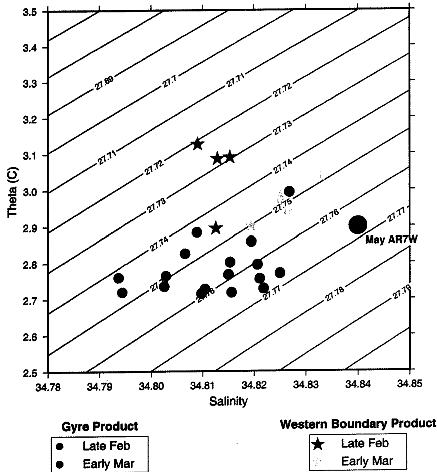
FIG. 14. Time evolution of mixed layer \theta - S between the two occupations of Section 2, for the gyre and boundary regions. The final springtime product (see text) is indicated by the large black circle.
