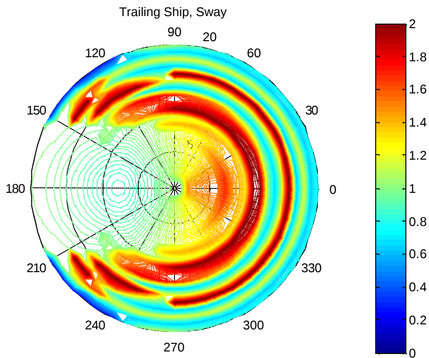
Figure A-357. SLICE Sway Amplitude Motion (HS: 30 feet, T_m : 20 sec., l/L : 1.0)
