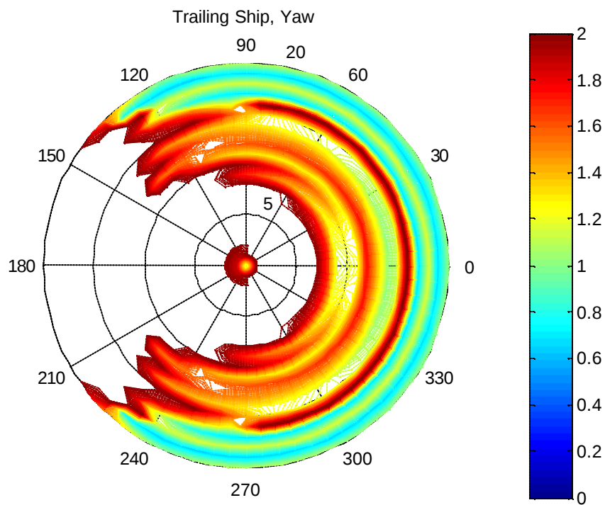
Figure A-359. SLICE Yaw Amplitude Motion (HS: 30 feet, T_m : 20 sec., l/L : 1.0)
