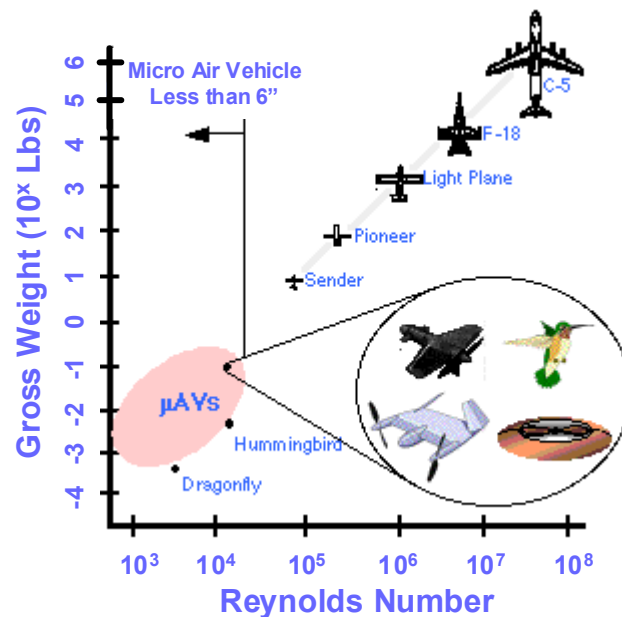
Figure 1 Comparison of the Micro Air Vehicle ( \mu AV) Flight Regime with Others 1
