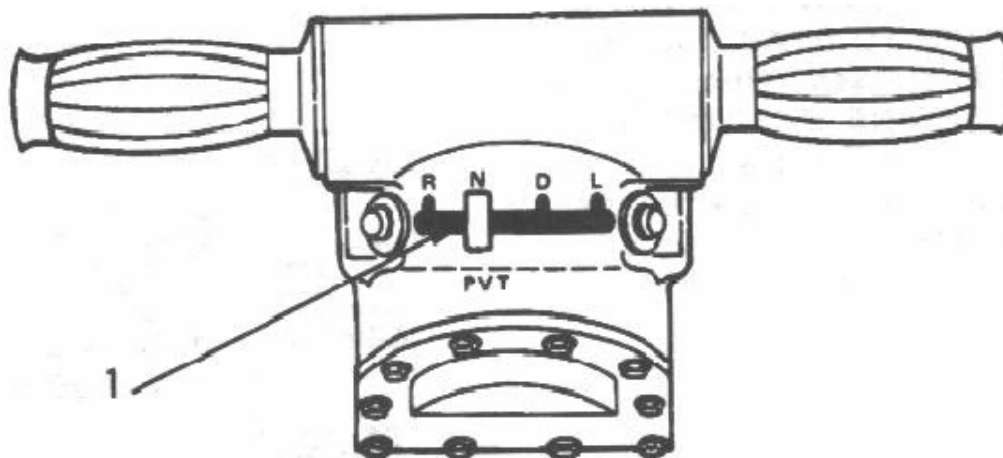
1 - Shift Control Selector
