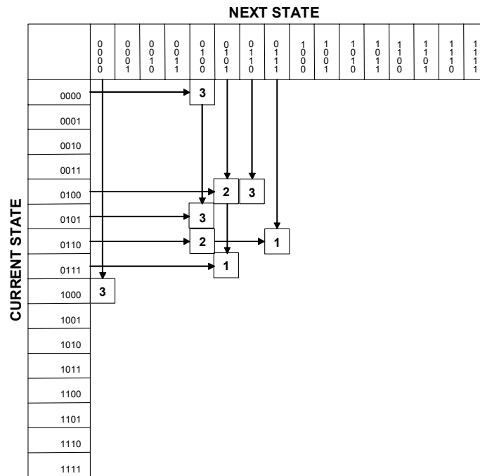
Figure 16. Sparse Matrix for Driver 3
