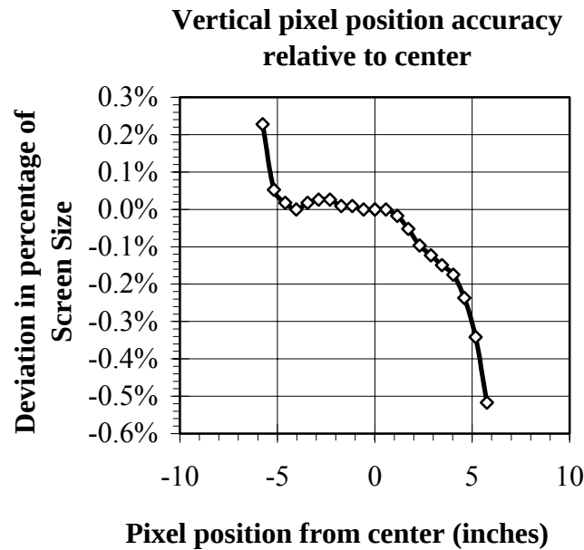
Fig. II.18-4 Vertical linearity characteristic for 1600 x 1200 x 72 Hz.
