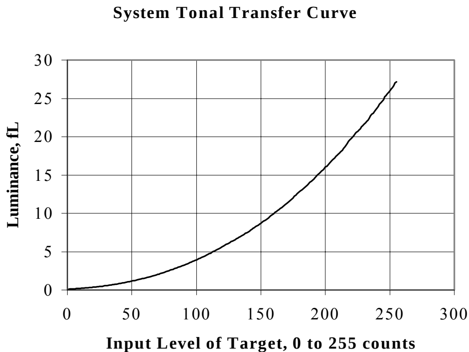
Figure II.6-1. System Tonal Transfer at center screen as a function of input counts.
