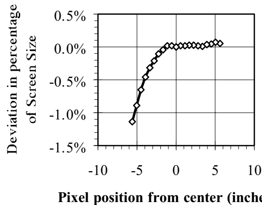
Fig. II.18-5 Horizontal and vertical linearity characteristics.
