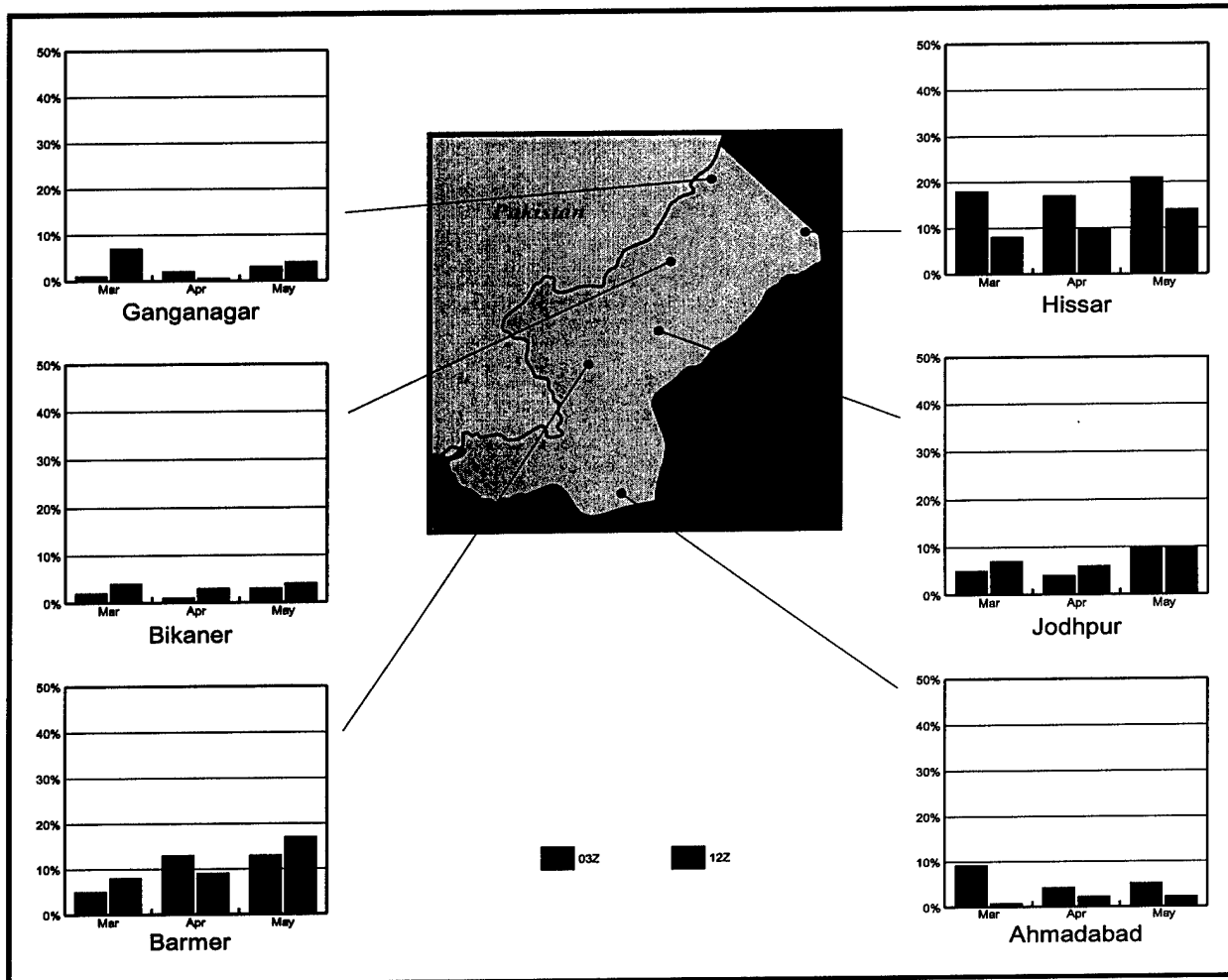
Figure 5-12. Hot Season Percent Frequency of Visibility below 2 1/2 Miles (4,000 Meters). The graphs show a monthly breakdown of the percent of visibility below 4,000 meters based on location and diurnal influences.
