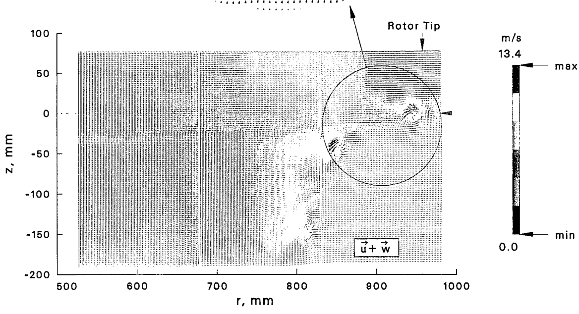
Figure 35: Enlargement of inplane velocity in zone A for \theta = 5^\circ and \psi = 12.4^\circ (2 chords).
